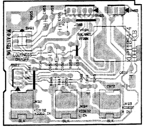
FRONT PCB-4 (LOUD PCB)
