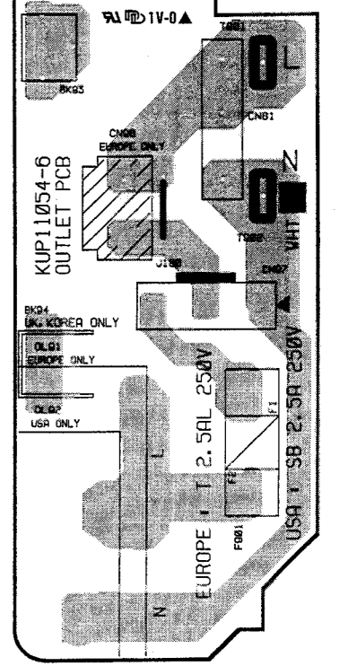
FRONT PCB-6 (OUTLET PCB)
