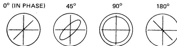
Fig. 5-4 Confirming phase relationship
