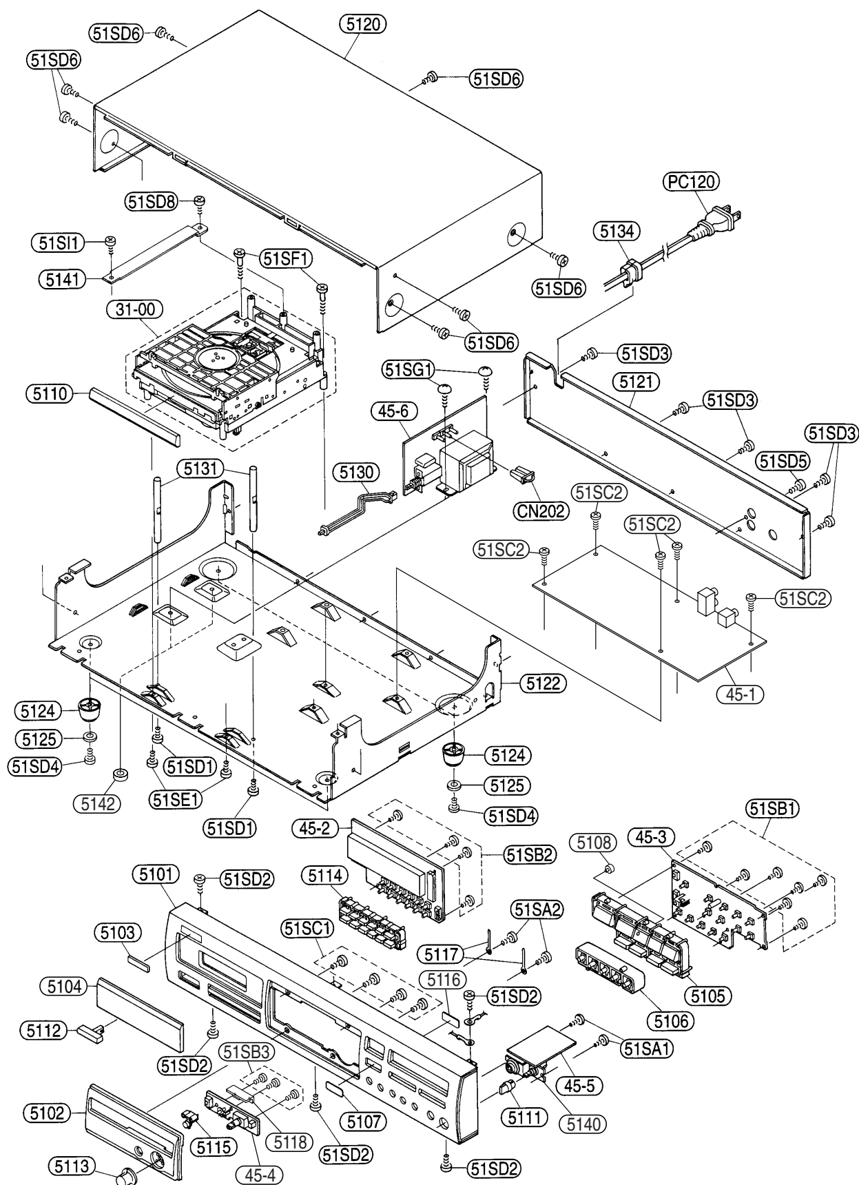
EXPLODED VIEW-1
