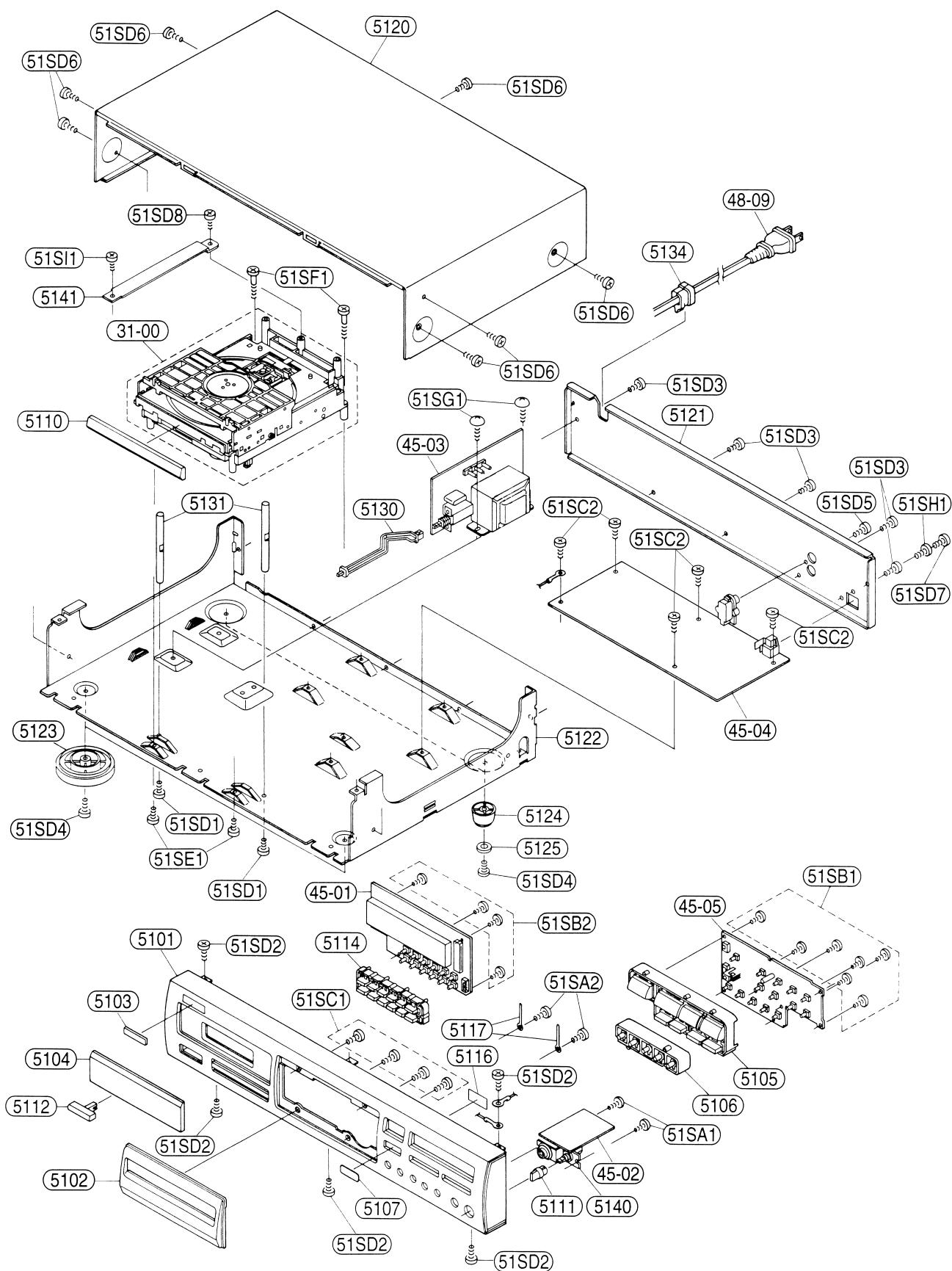
EXPLODED VIEW-1
