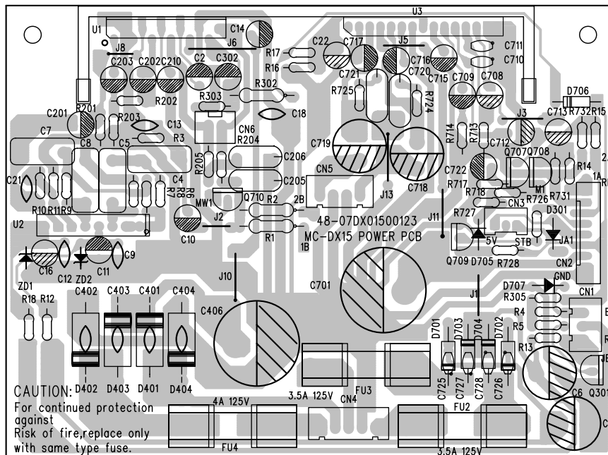
SUBWOOFER POWER PCB
