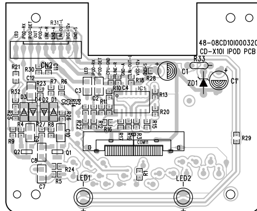
IPOD PCB
