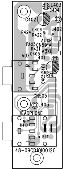
HP/AUX JACK PCB
