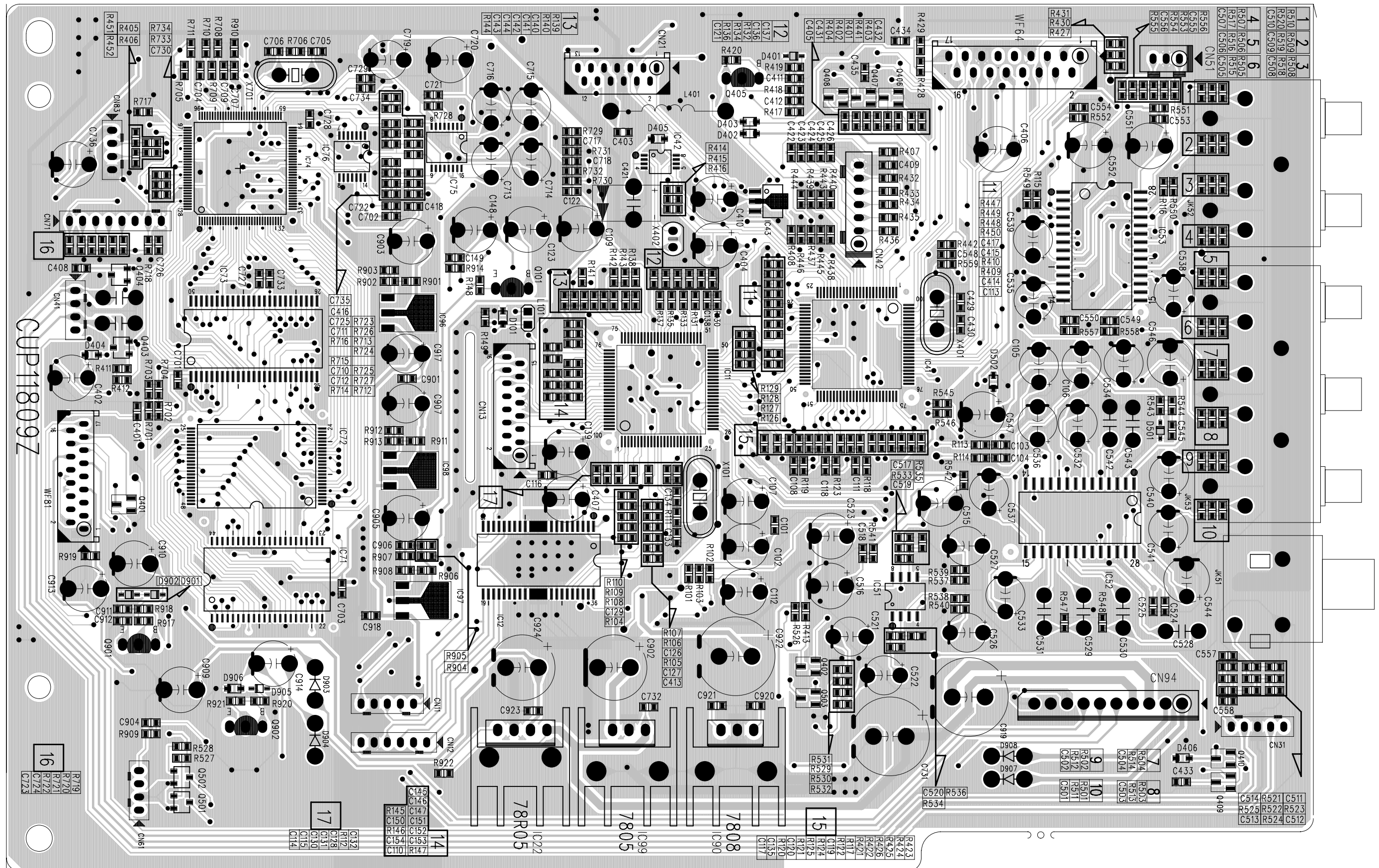
MAIN PCB (TOP VIEW)
