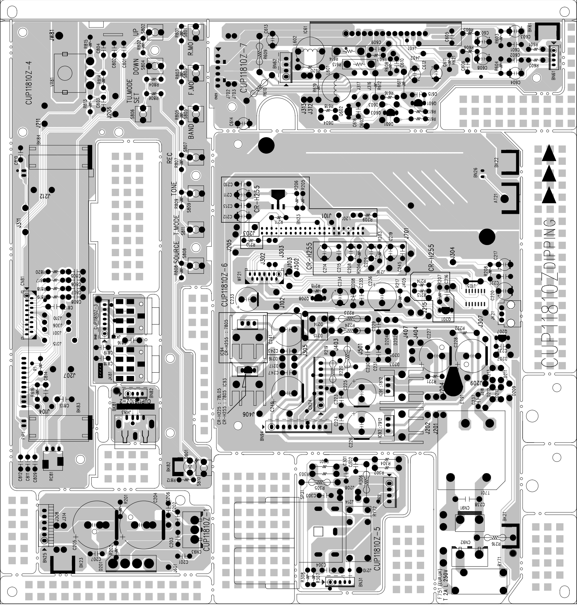
POWER PCB (TOP VIEW)
