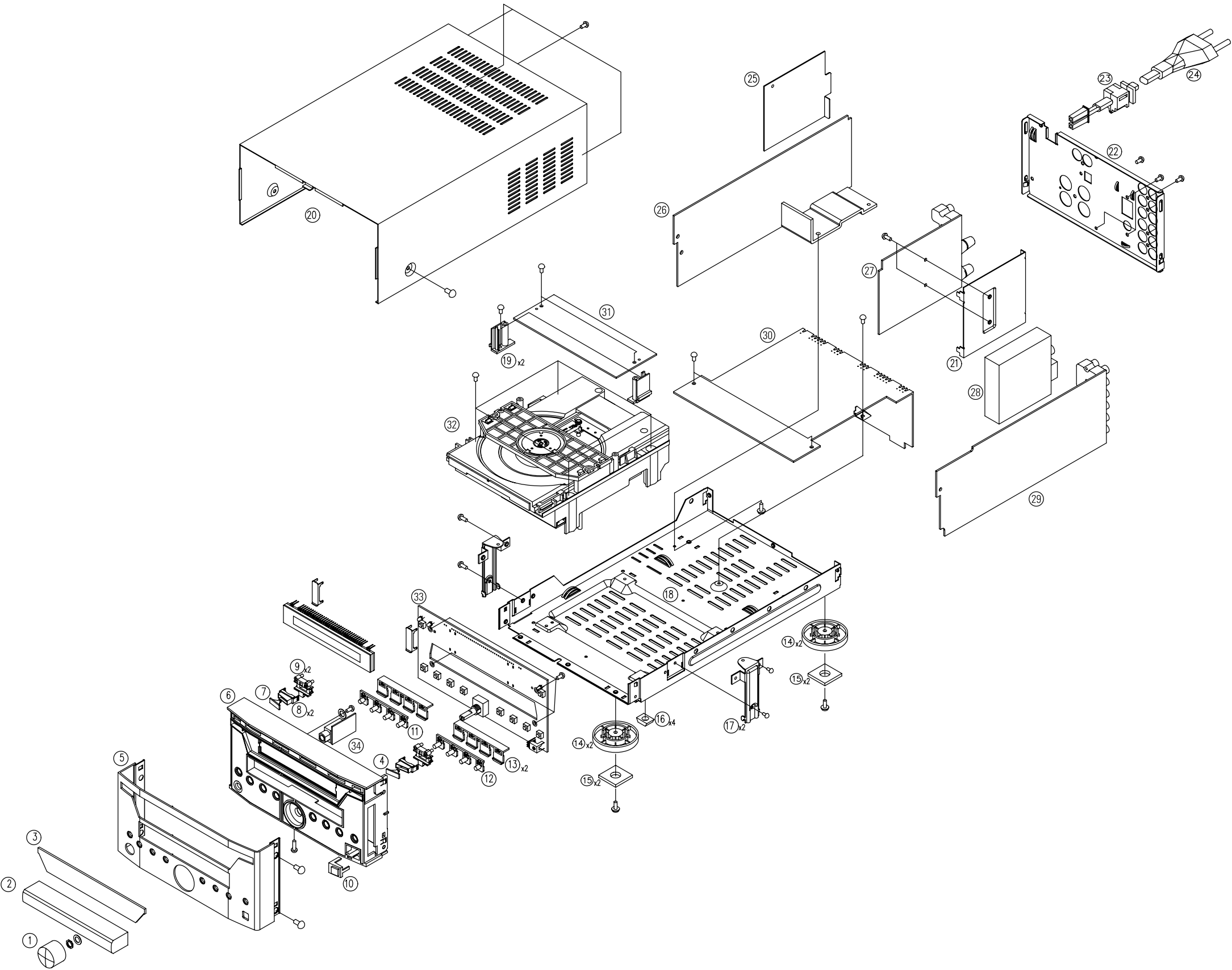
EXPLODED VIEW-1
