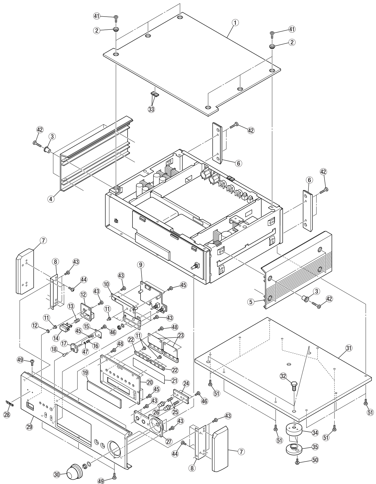
EXPLODED VIEW-1
