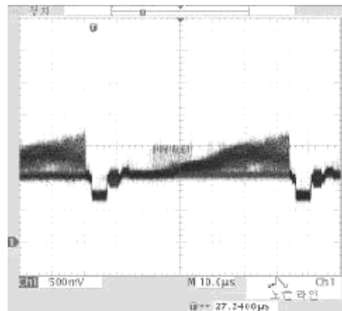
20. COMPOSITE-OUT
