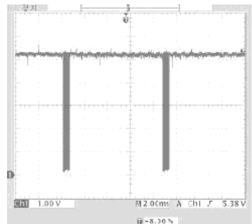
4. I2C-CLK
