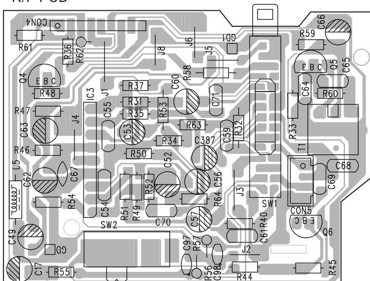
R/P PCB
