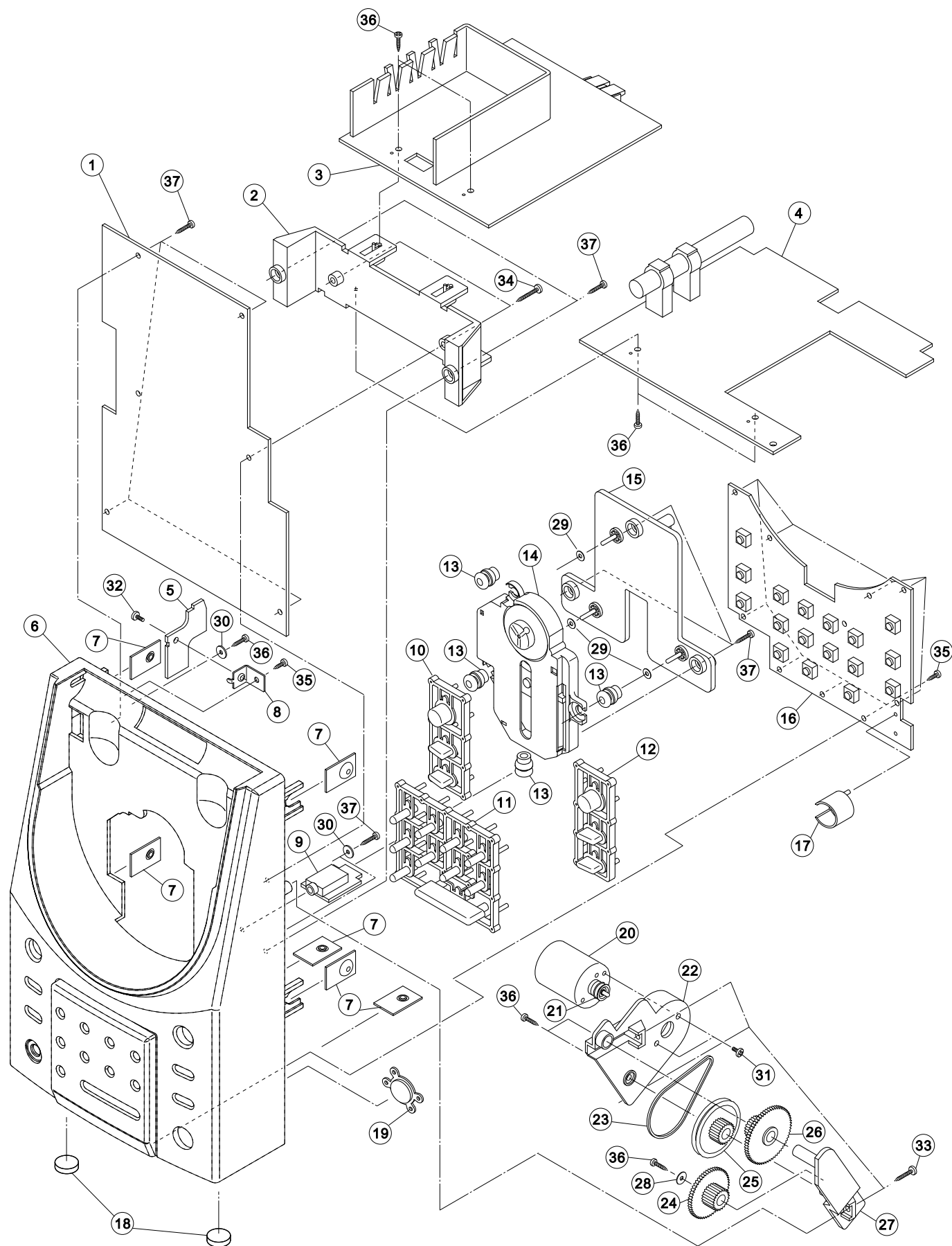
EXPLODED VIEW - 1
