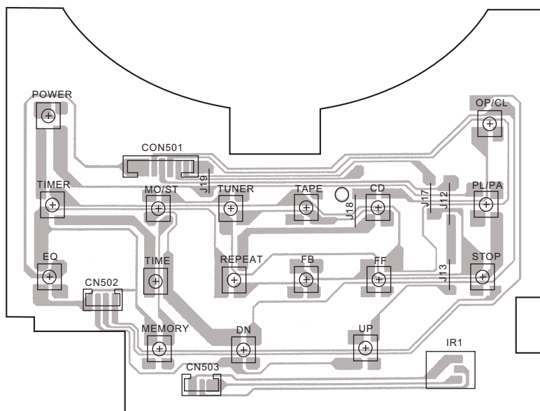
KEY PCB
