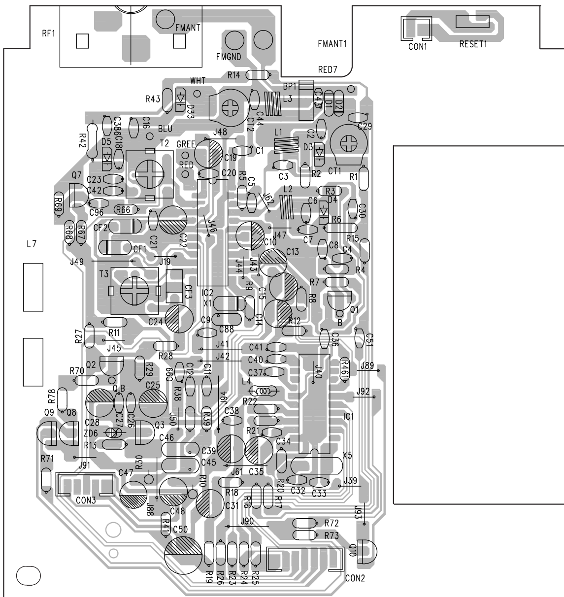
TUNER PCB
