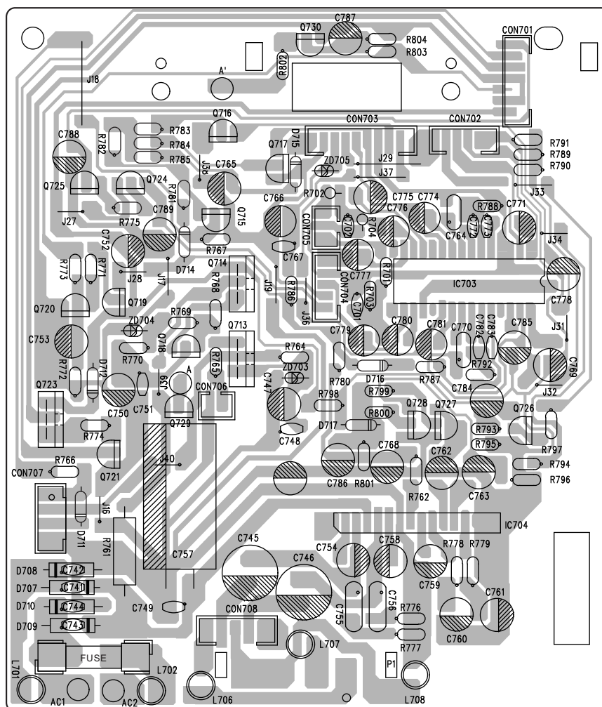
POWER PCB
