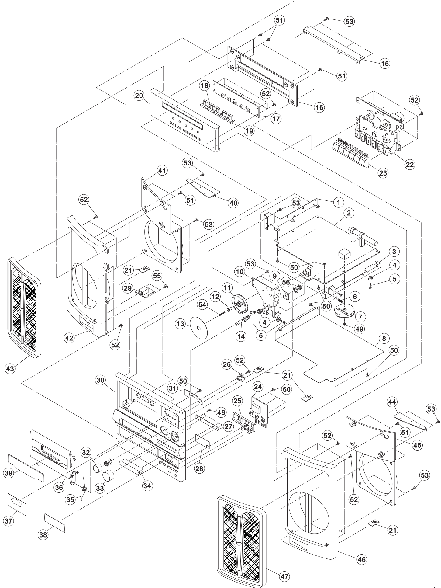
EXPLODED VIEW - 1
