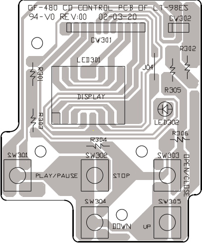
CONTROL PCB
