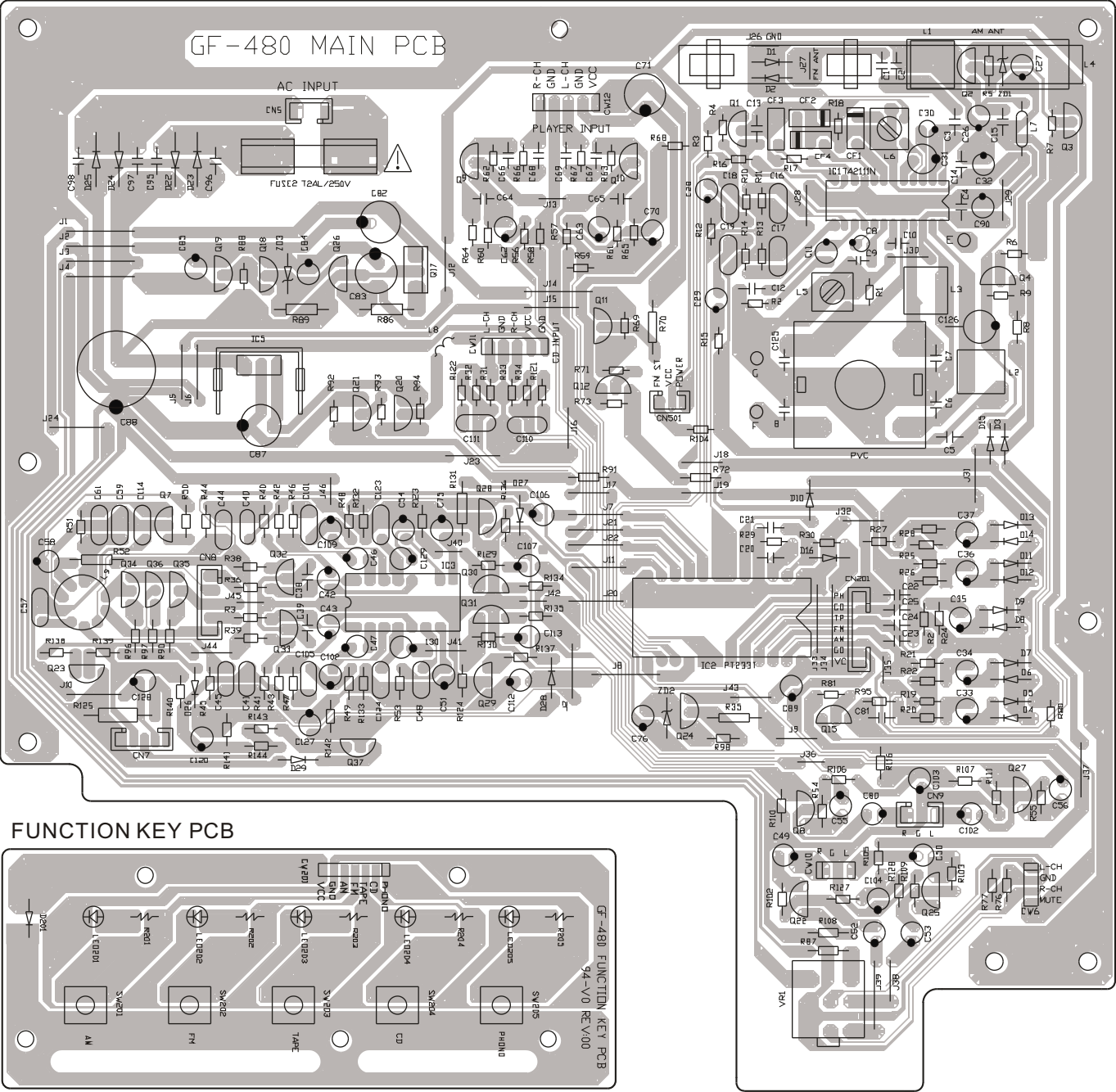
MAIN PCB
