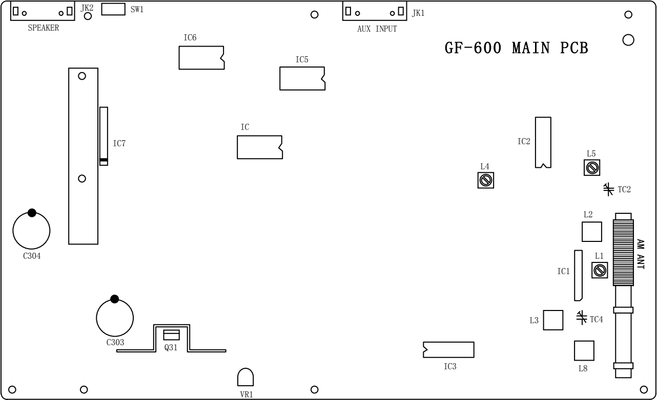
FIG 3-9 Adjustment locations
