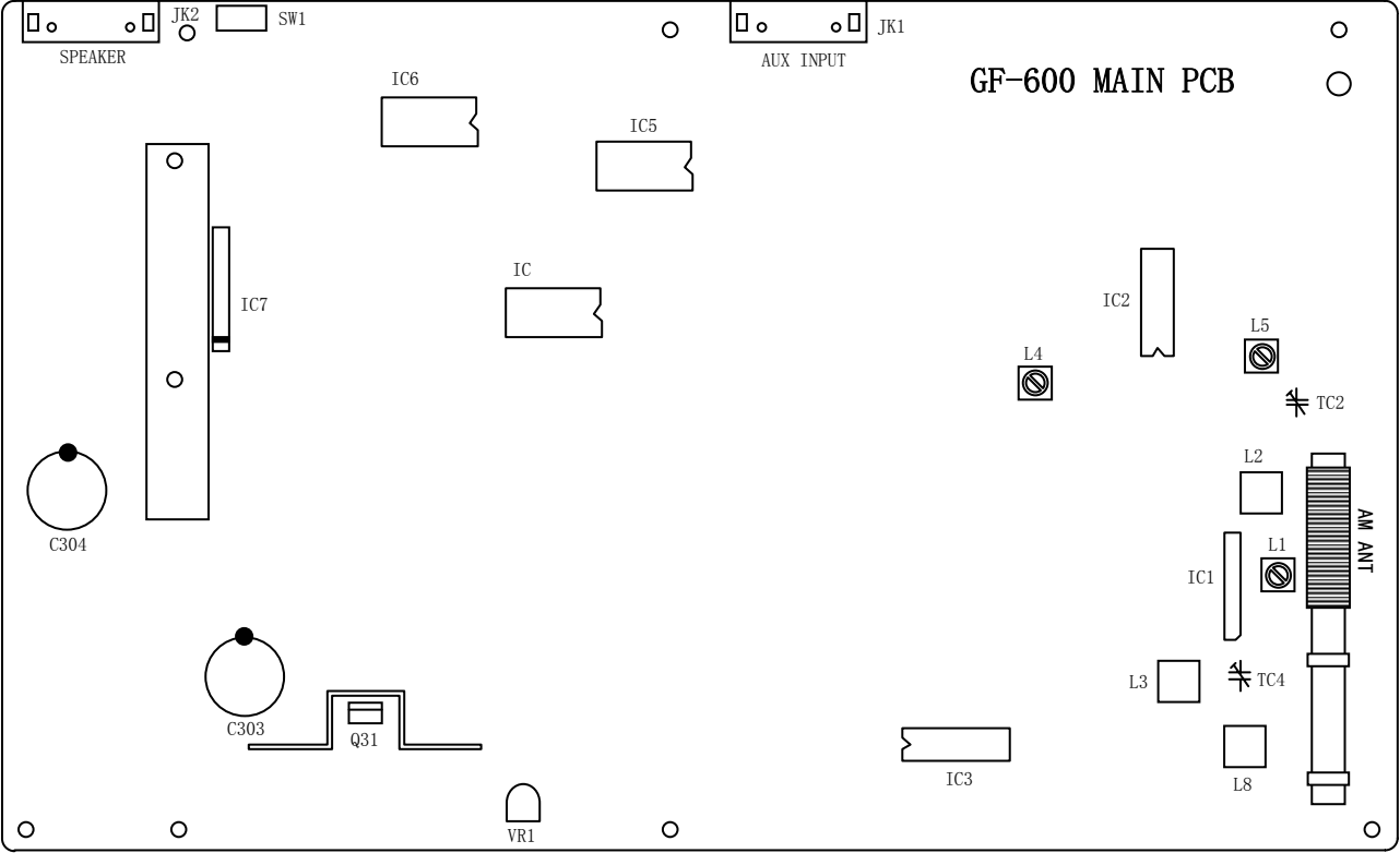
FIG 3-2 Adjustment locations
