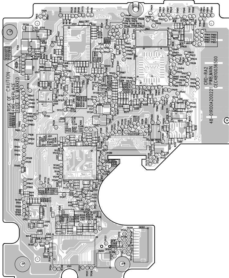
POWER MAIN PCB (CD MECHAN. ASSY) - BOTTOM
