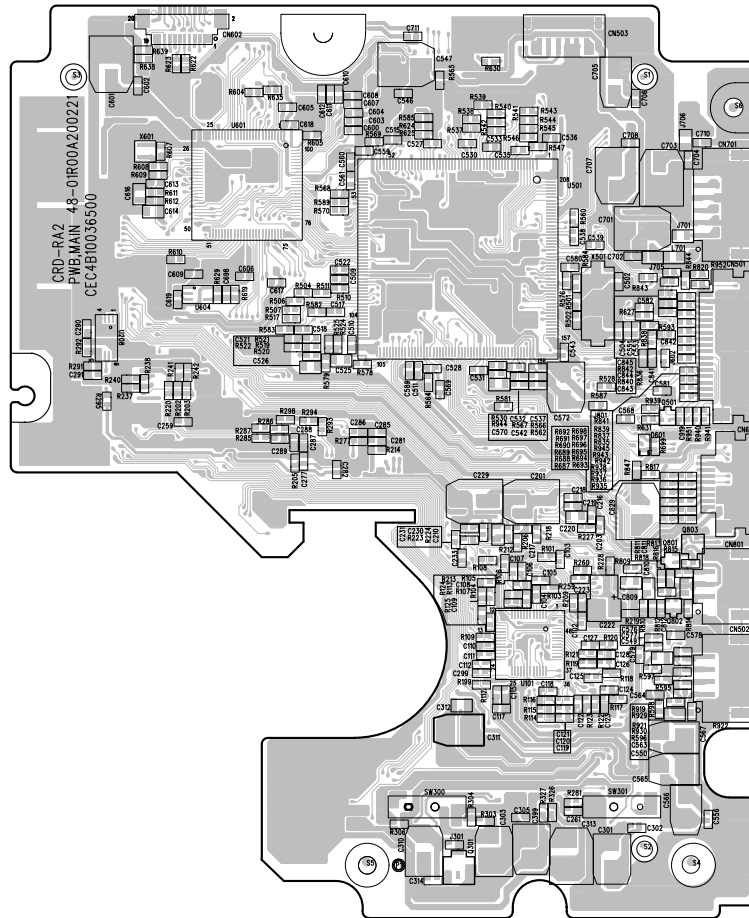
POWER MAIN PCB (CD MECHAN. ASSY) - TOP
