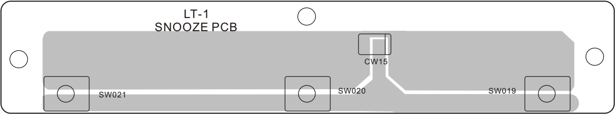
SNOOZE PCB
