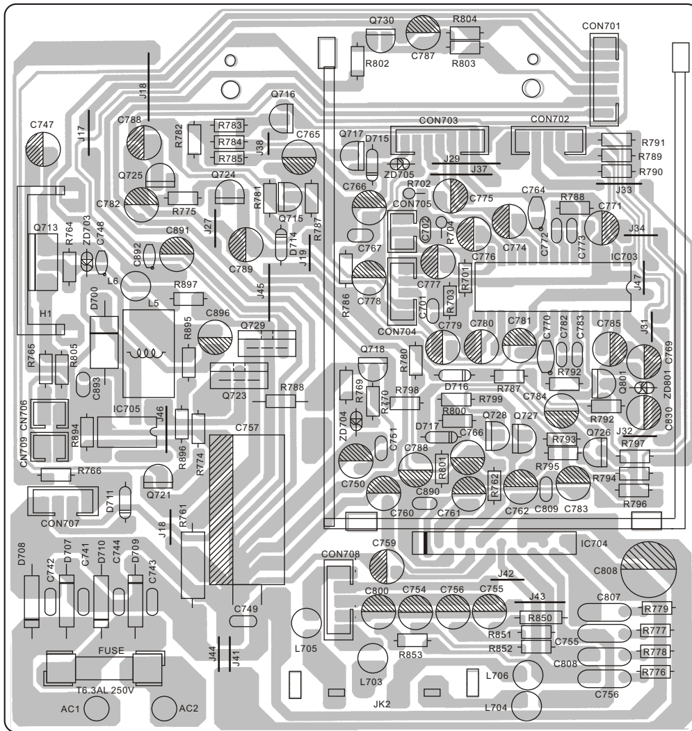
POWER PCB
