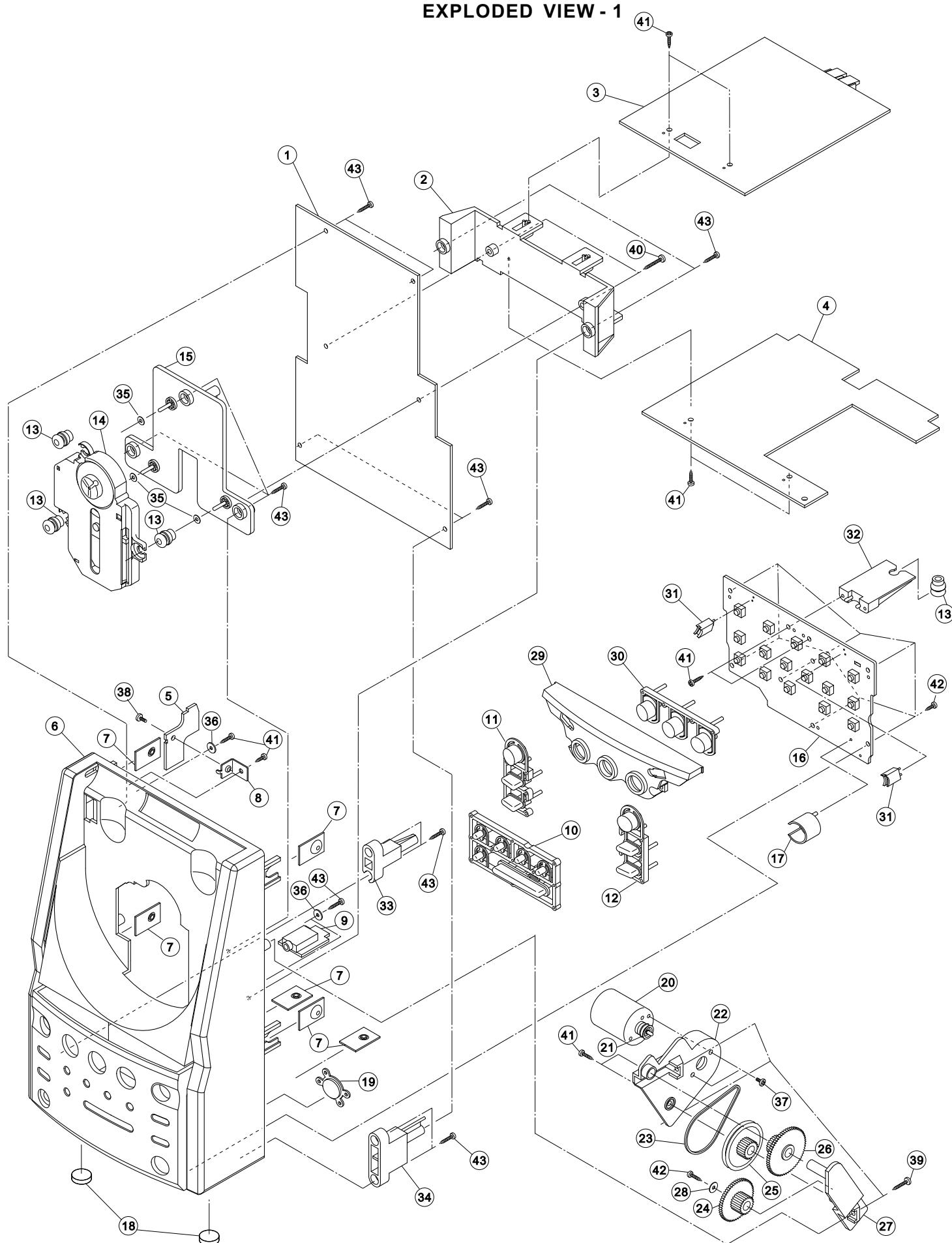
EXPLODED VIEW - 1
