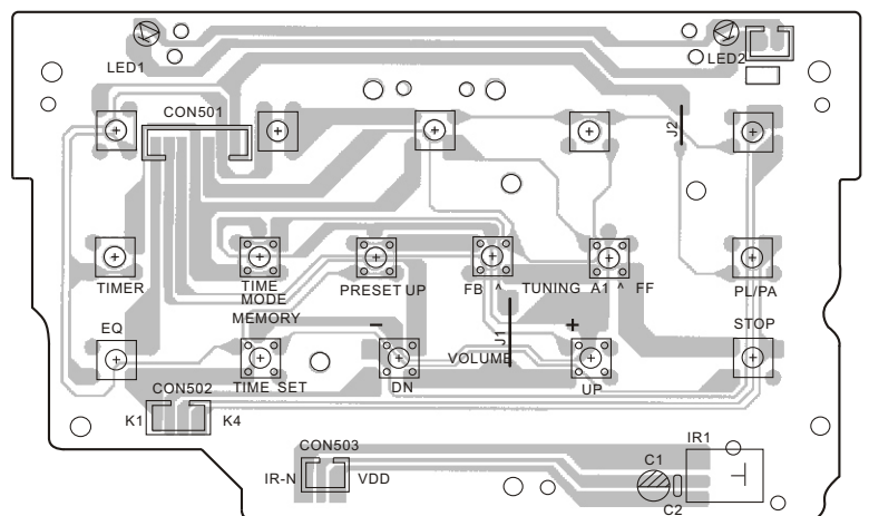
KEY PCB
