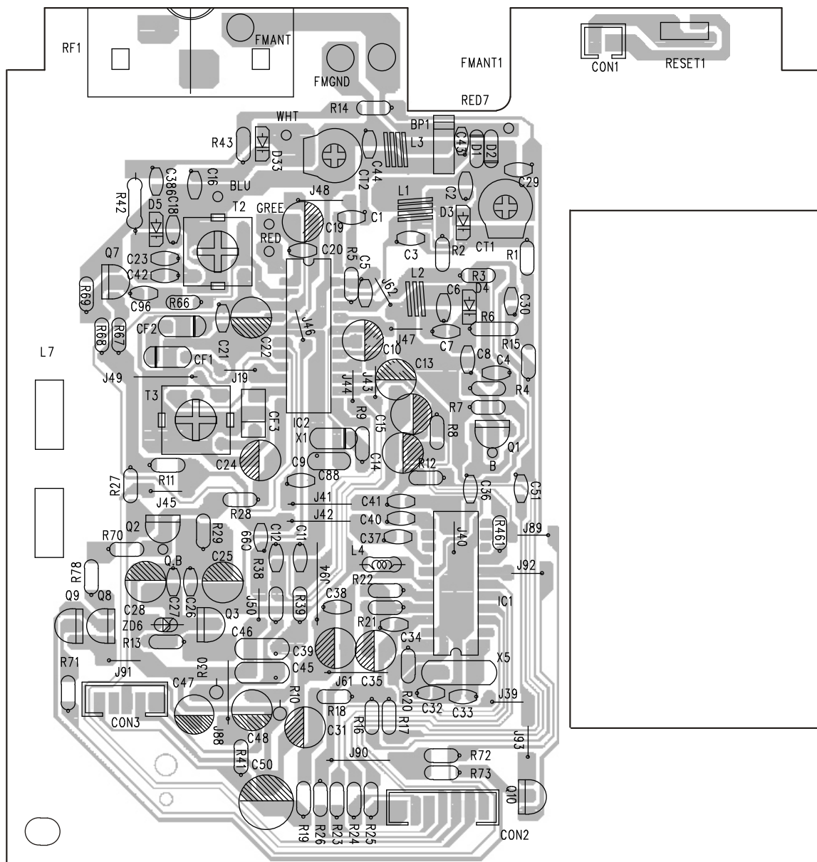
TUNER PCB
