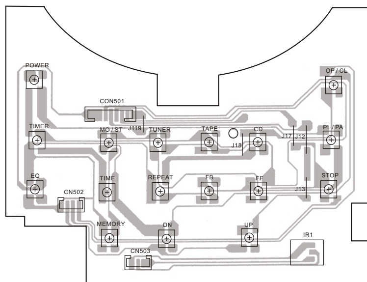
KEY PCB
