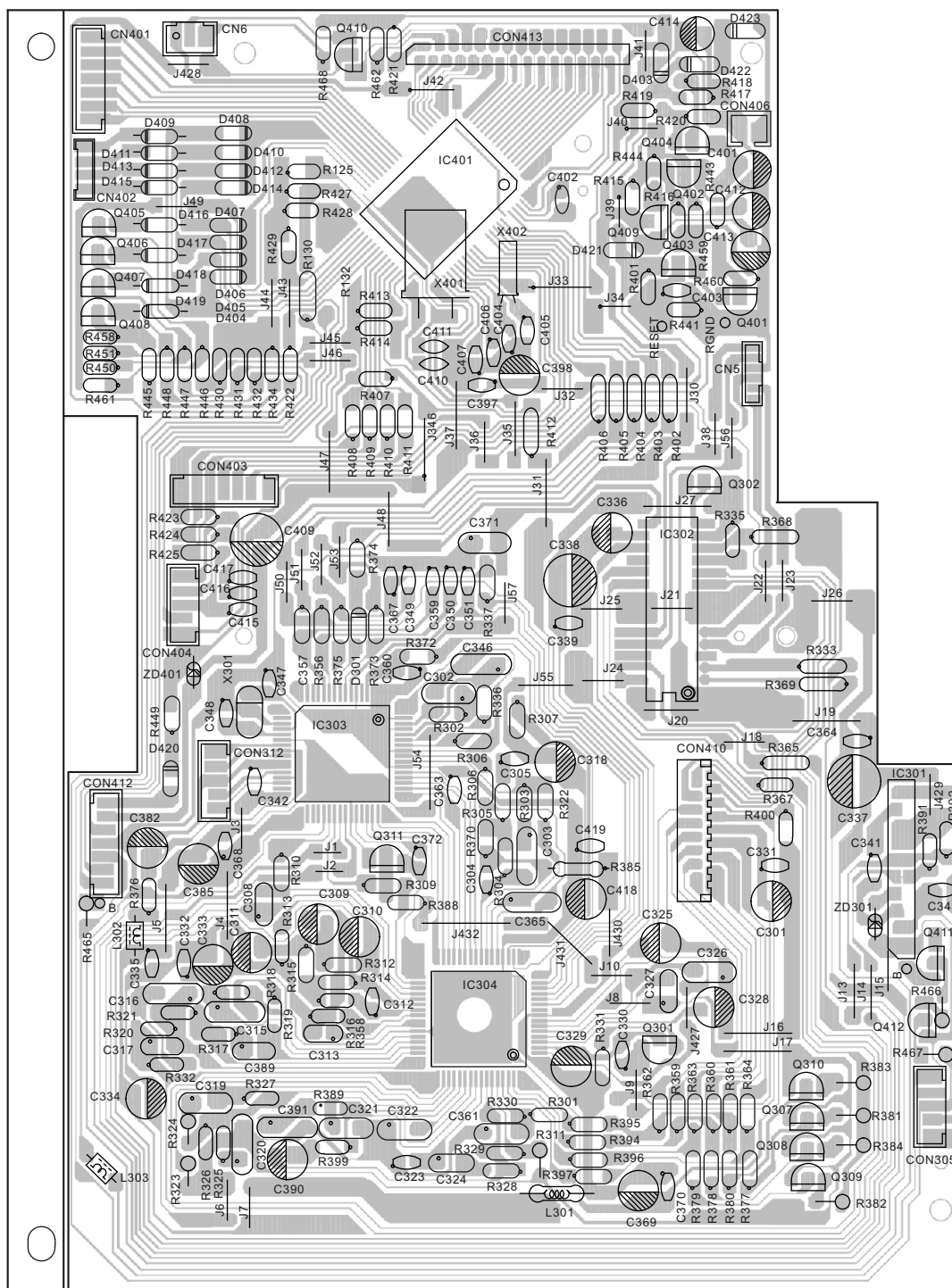
CD PCB
