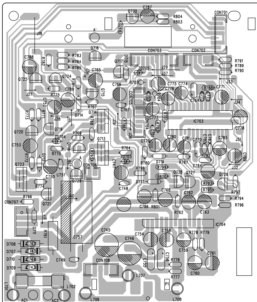
POWER PCB
