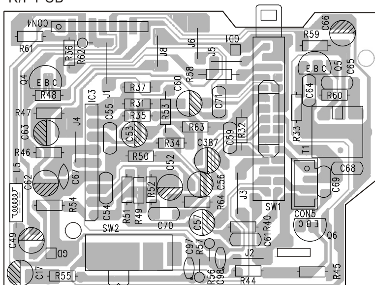
R/P PCB
