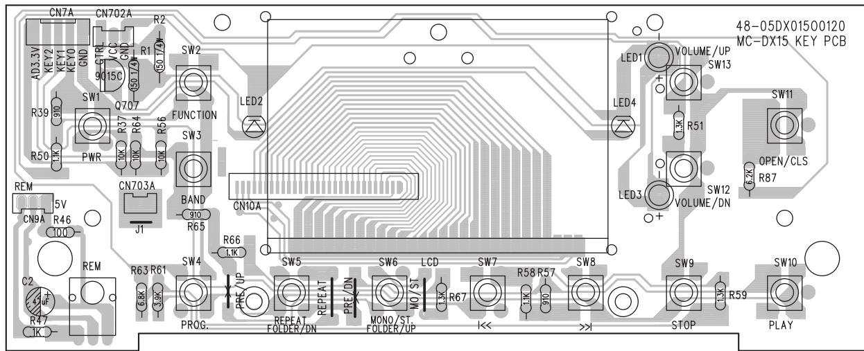
KEY/DISPLAY PCB
