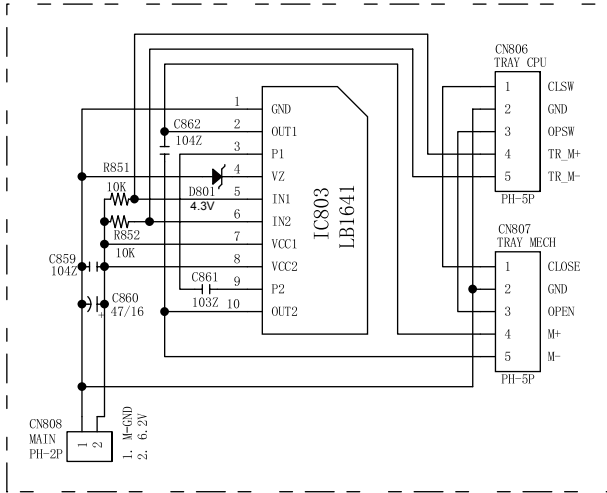
Option for Front-Loading Mechanism
