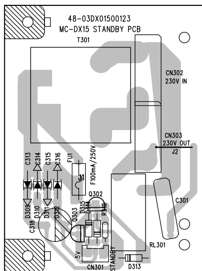
STANDBY PCB
