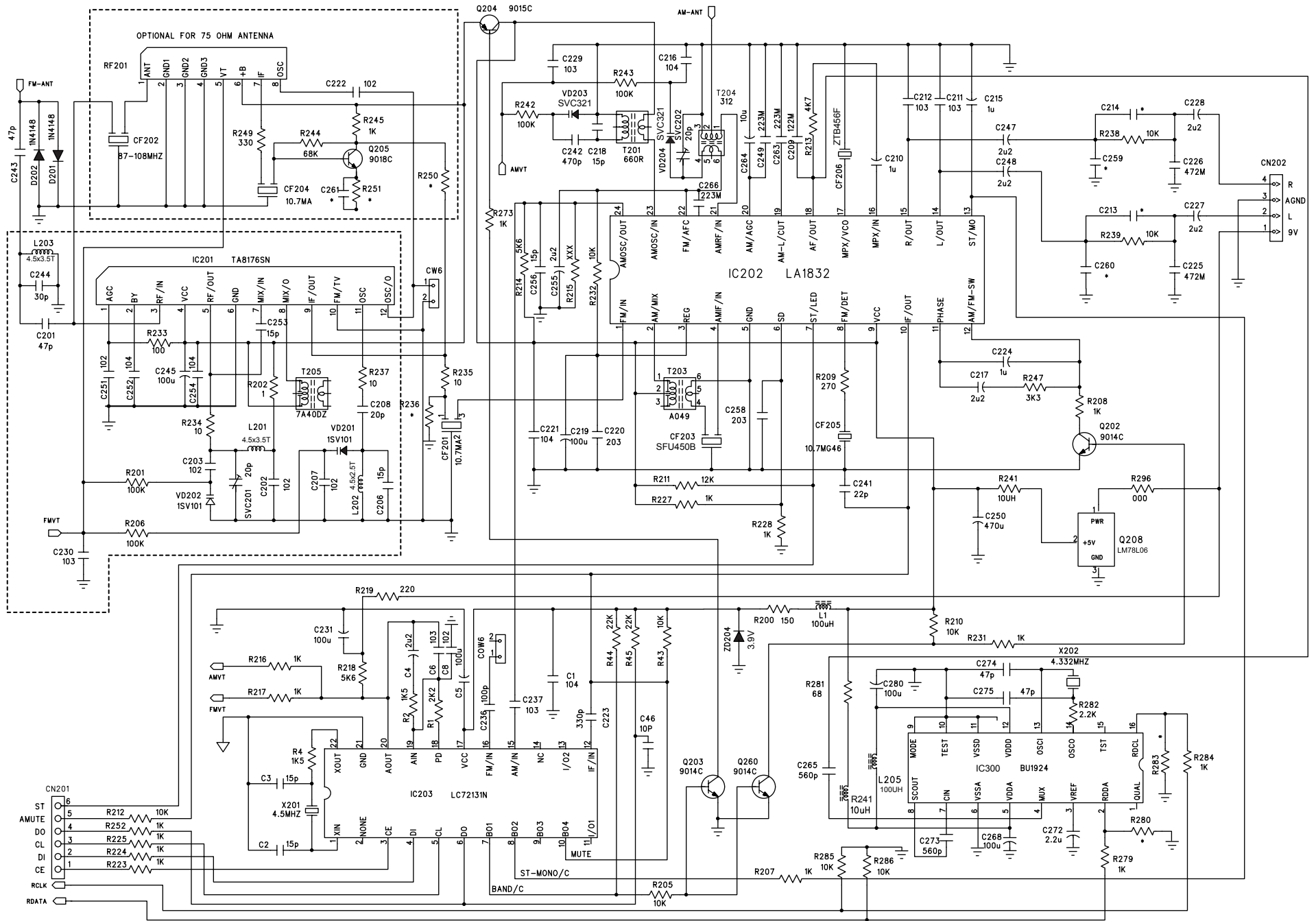
MC-DX220i/MC-DX22i Micro Hi-Fi System
