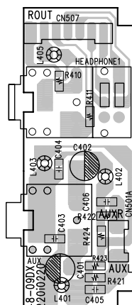
HEADPHONE PCB
