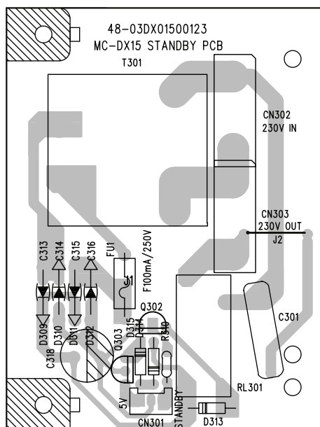
STANDBY PCB
