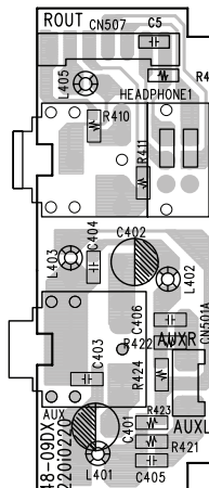
HEADPHONE PCB
