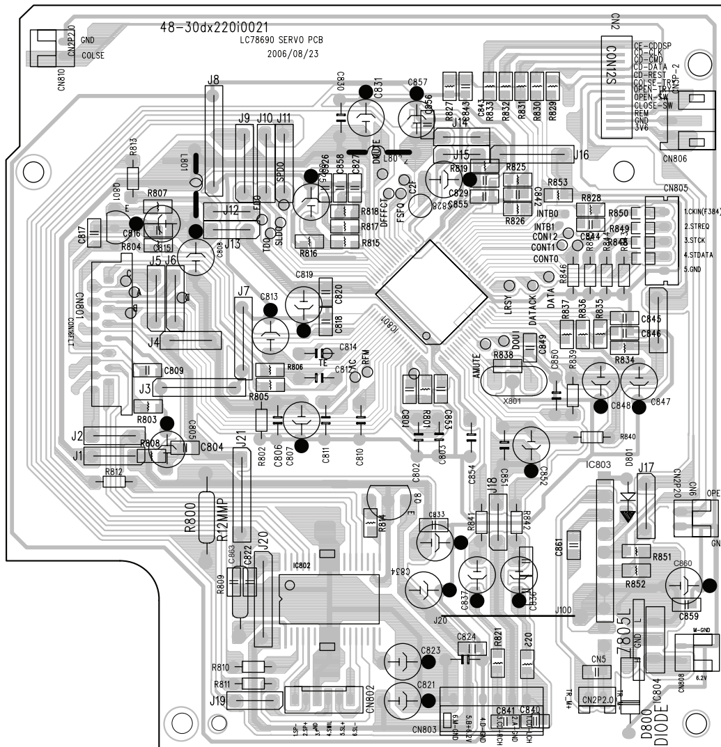
CD PCB
