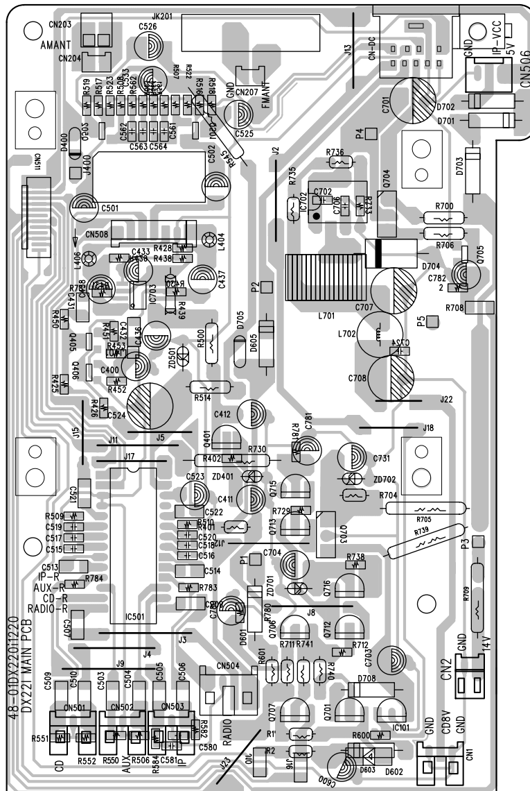
MAIN PCB
