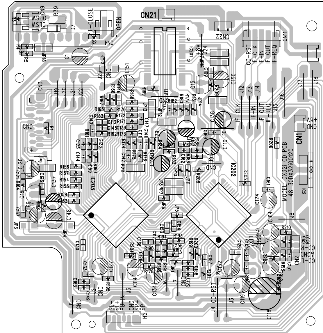
CD PCB
