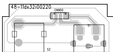
TV PCB
