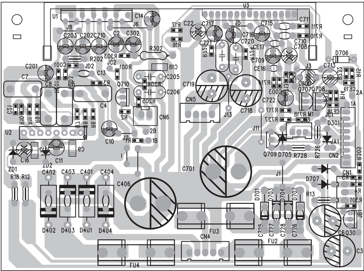
POWER PCB
