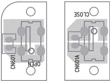
SWITCH PCB
