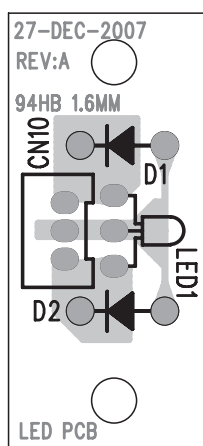
LED PCB
