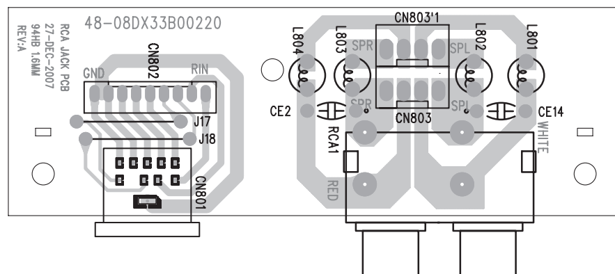
RCA JACK PCB
