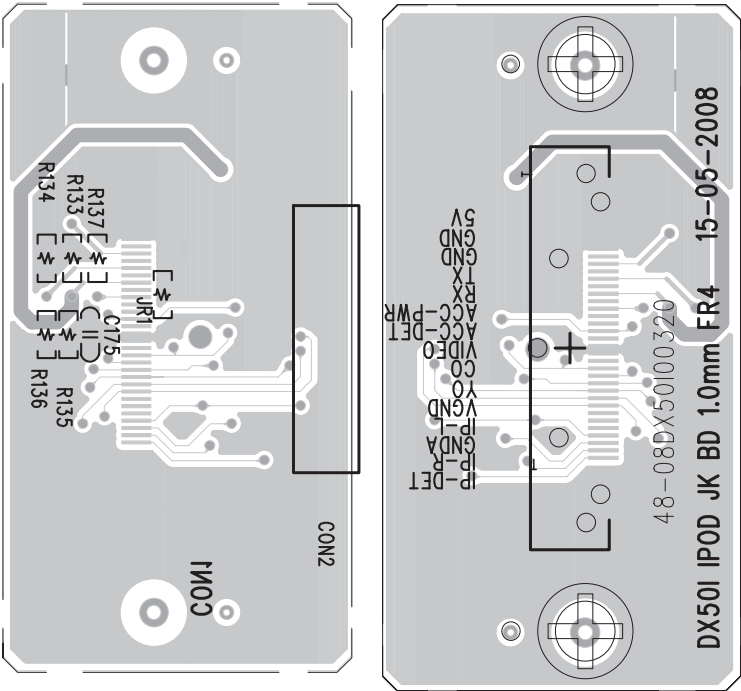
IPOD PCB
