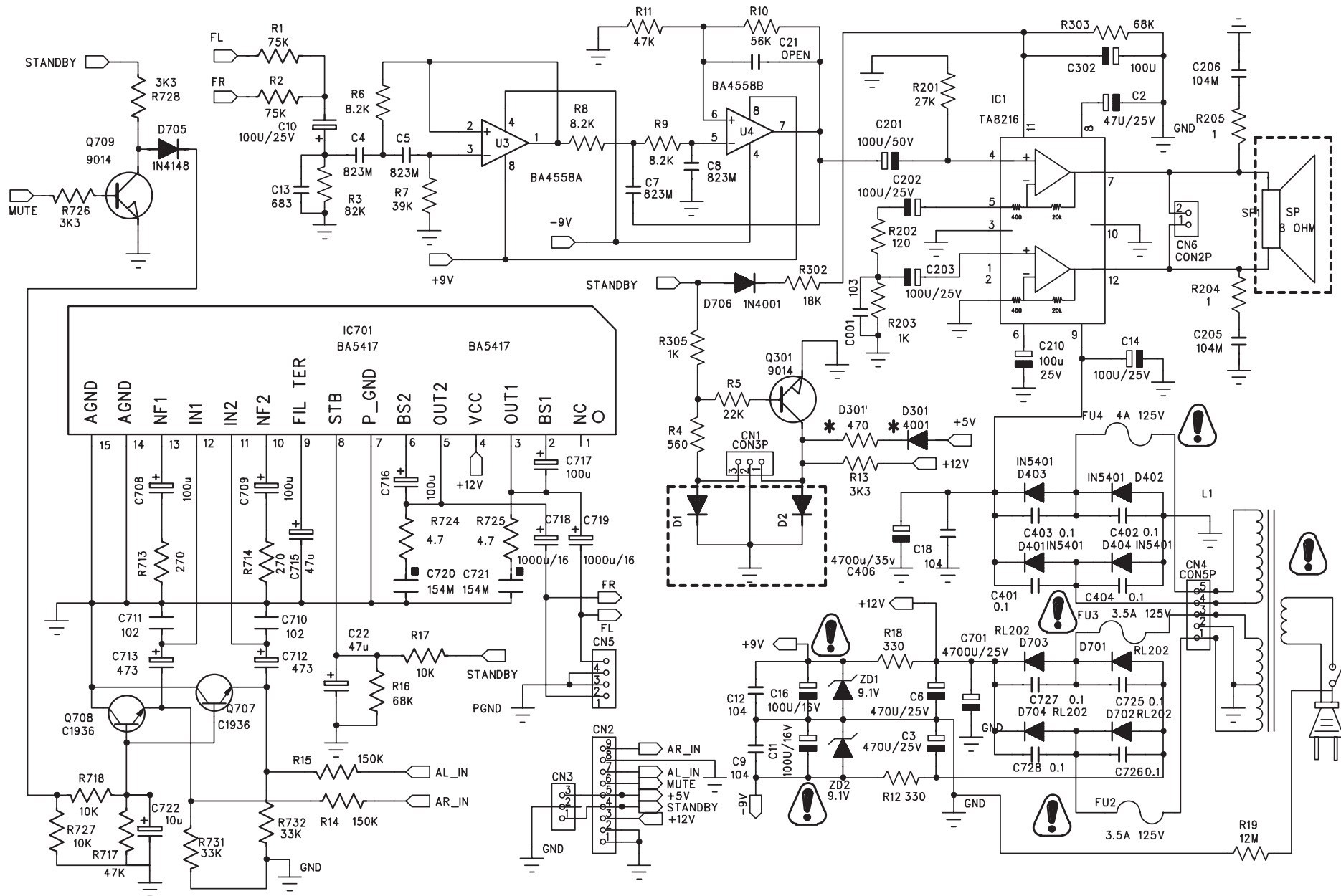
MC-DX50i Micro Hi-Fi system
