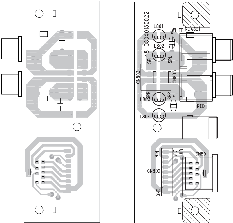
RCA JACK PCB
