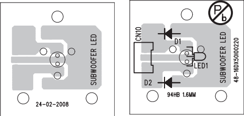
SUBWOOFER LED PCB
