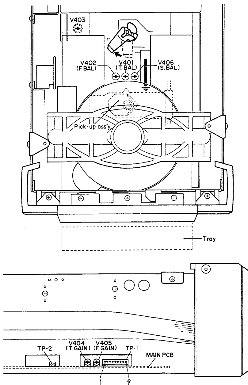
Fig.4-3 Adjustment location
