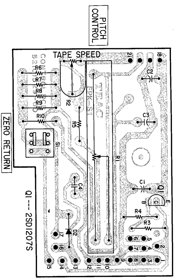
CONTROL PCB ASS'Y
