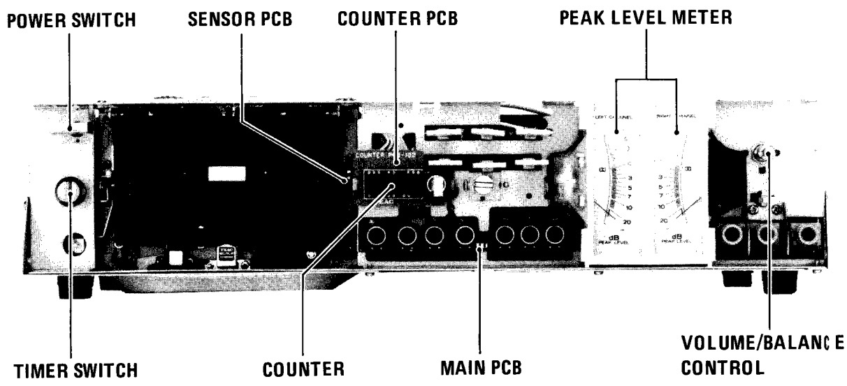
Fig. 3-2 Front view
