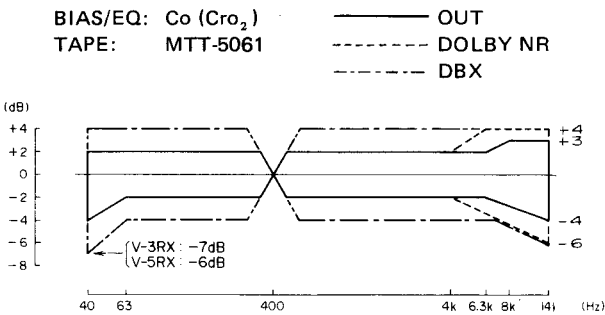
Fig. 5-8 Overall frequency response [Co (CrO 2 )]
