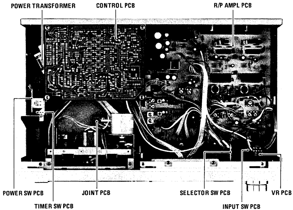
Fig. 3-1 Top view
