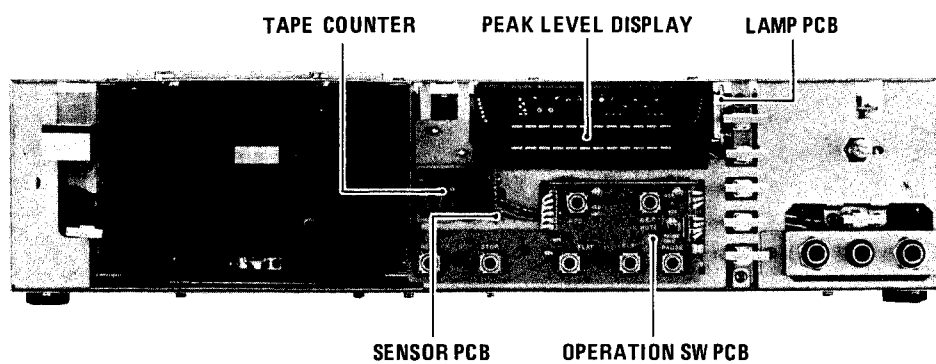
Fig. 3-2 Front view
