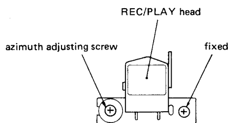
Fig. 5-4 Azimuth screw location
