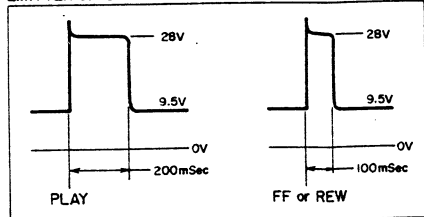
EMITTER OF Q733
