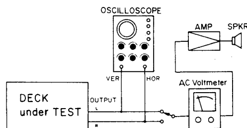
Fig. 4-6 Test setup for azimuth check
