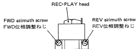
Fig. 5-4 Azimuth screw location 位相調整ネジ
