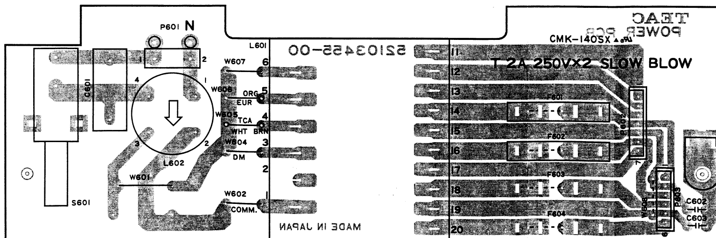
POWER PCB
