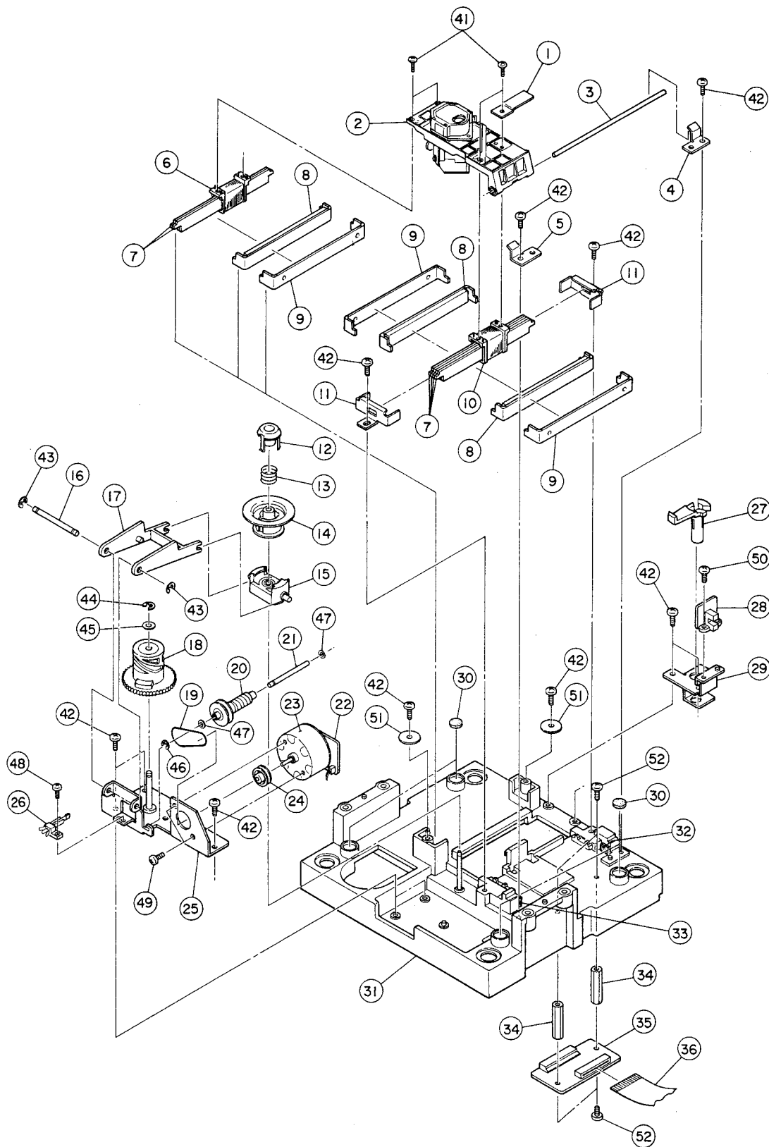
EXPLODED VIEW-3
