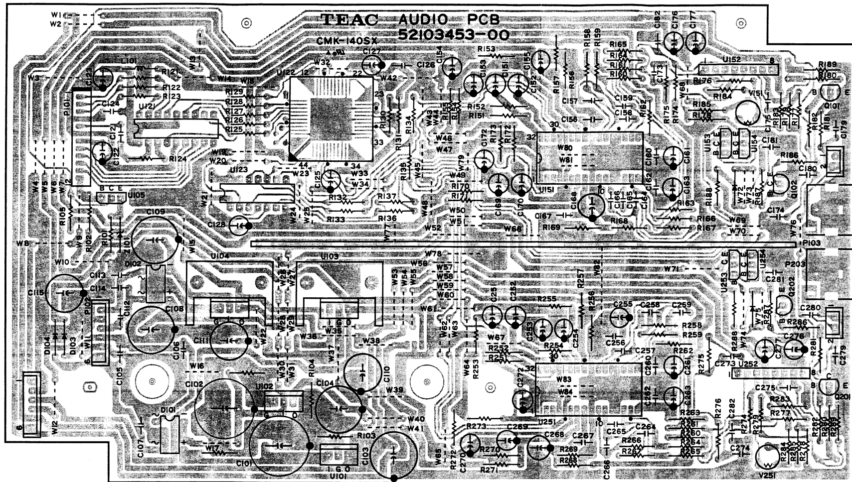
AUDIO PCB
