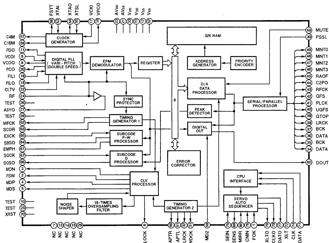
U403 CXD2500AQ
