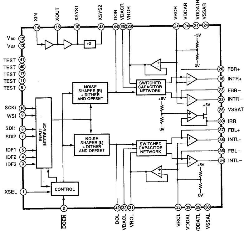
U122 SAA7350GP
