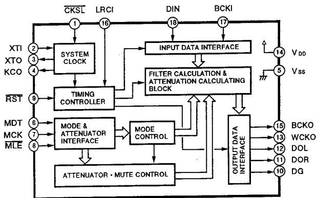
U121 SM5840AP
