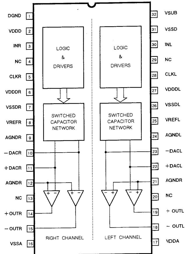
U151, 251 TDA1547
