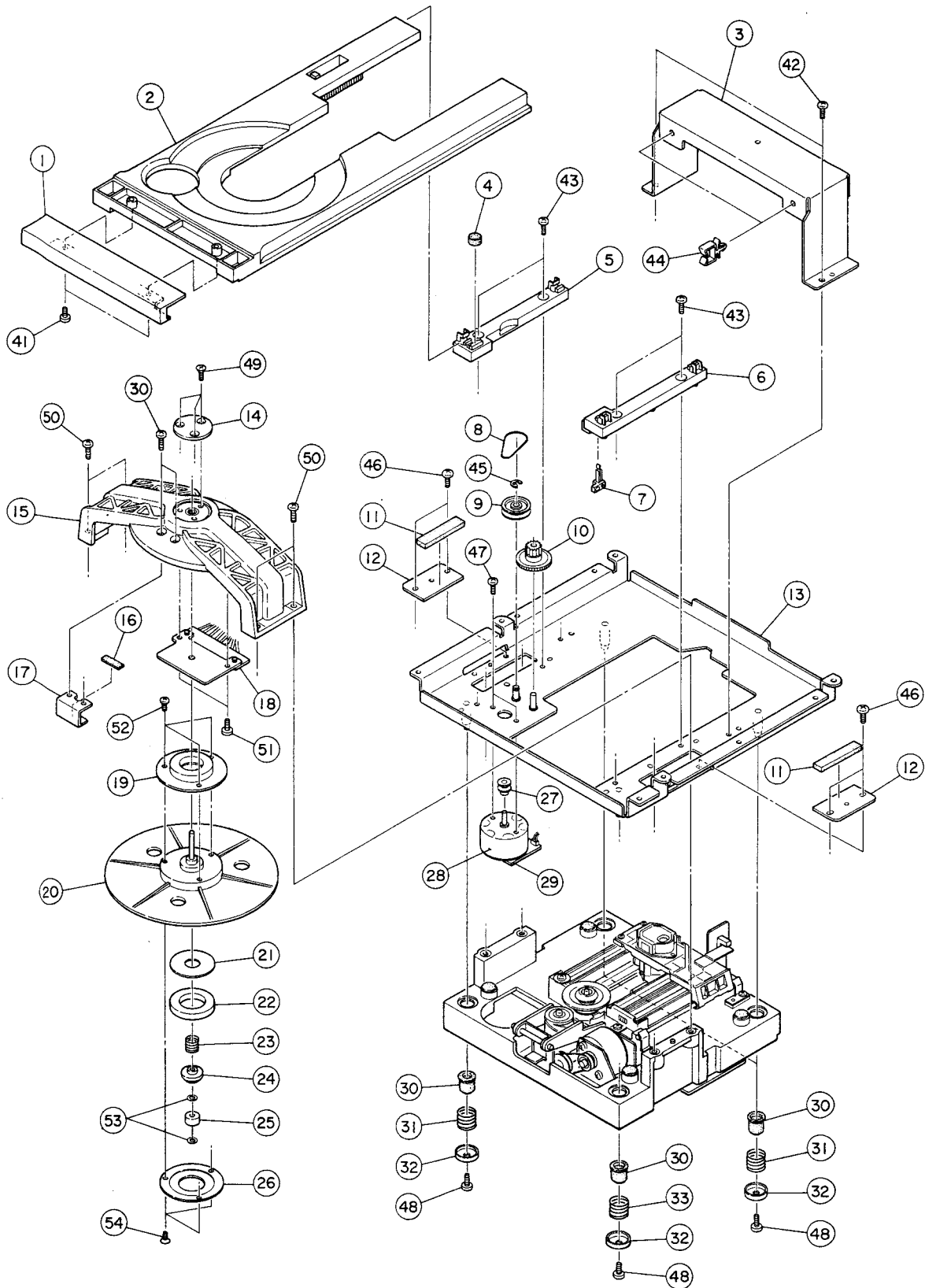
EXPLODED VIEW-2
