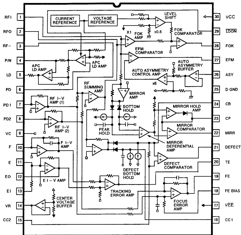
U401 CXA1081S
