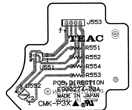
DIRECTION PCB
