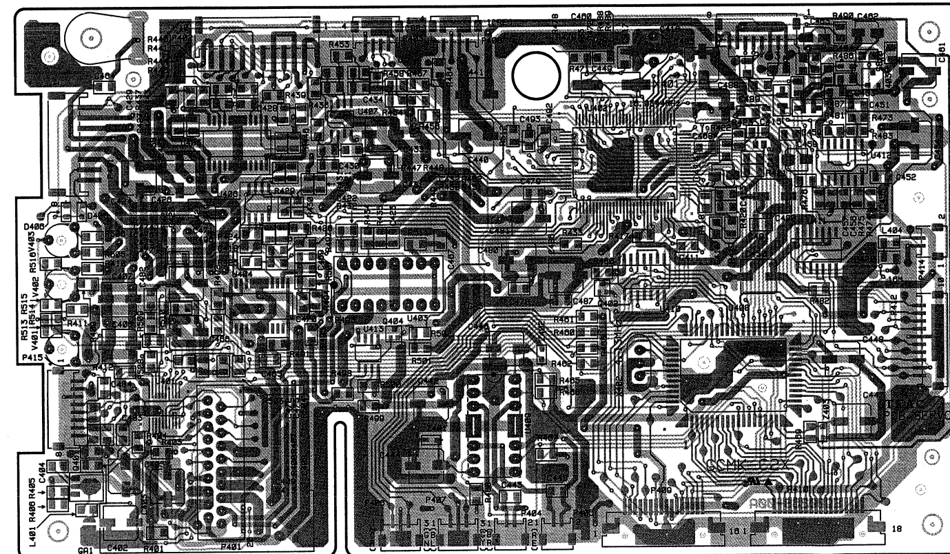
SERVO PCB
