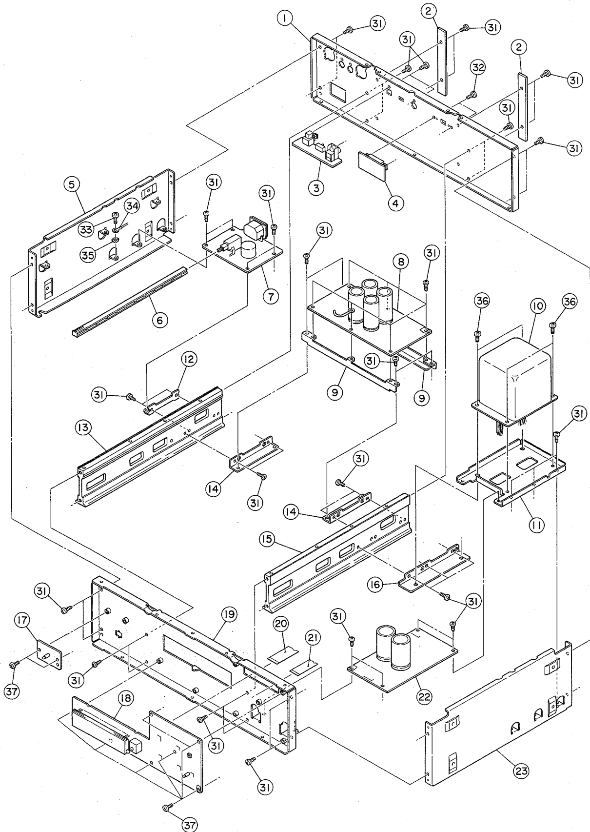
EXPLODED VIEW-2
