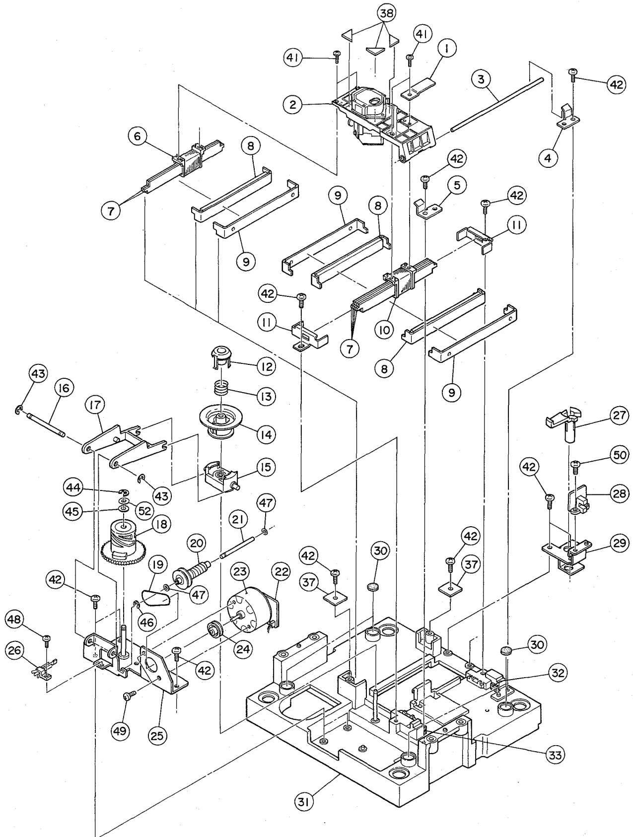
EXPLODED VIEW-4
