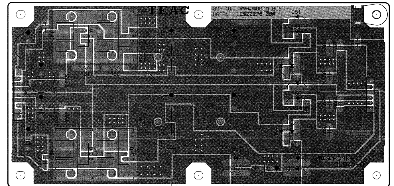
PWR-AUDIO PCB
