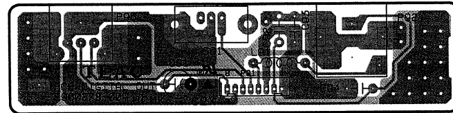
DIGITAL OUT PCB
