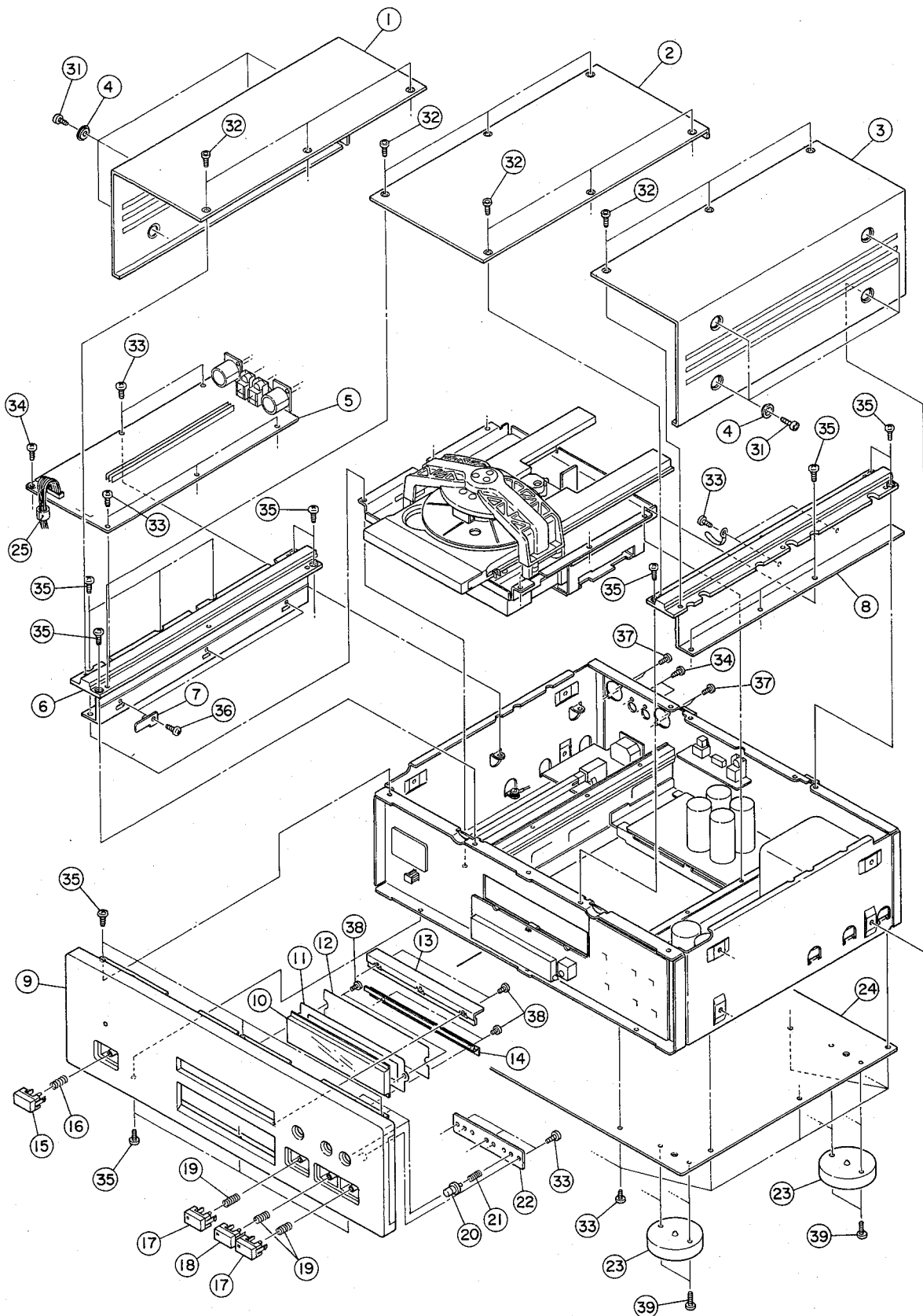
EXPLODED VIEW-1
