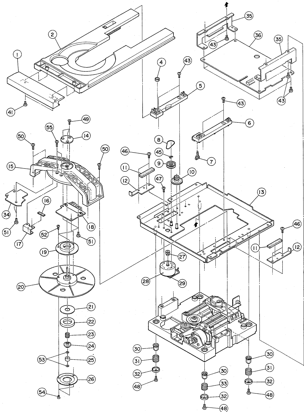
EXPLODED VIEW-3
