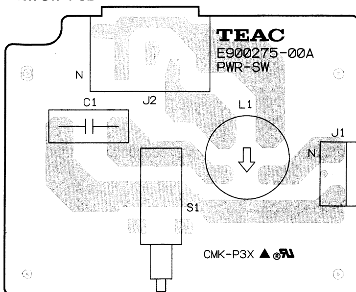
PWR-SW PCB
