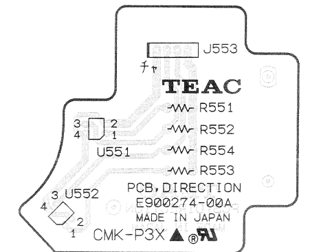
DIRECTION PCB
