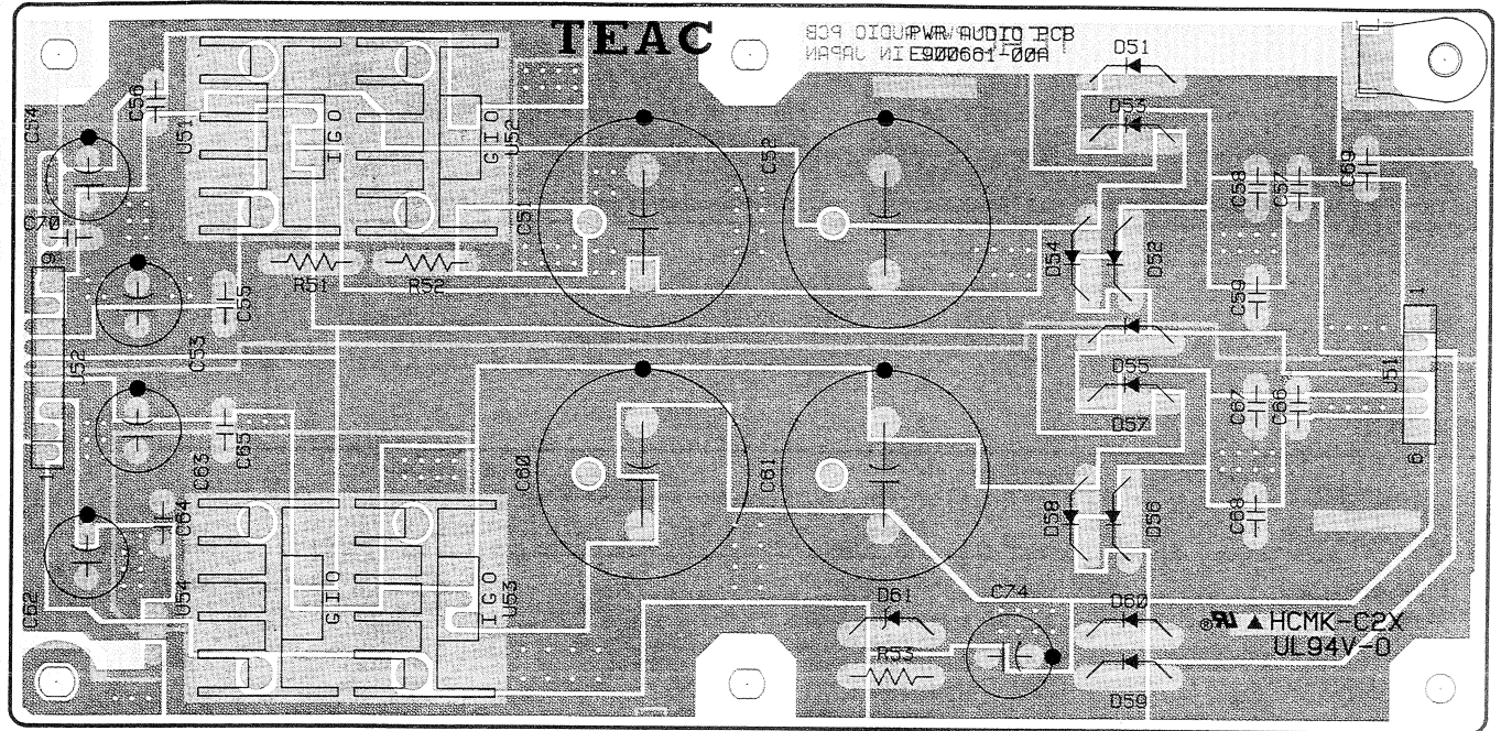
PWR-AUDIO PCB
