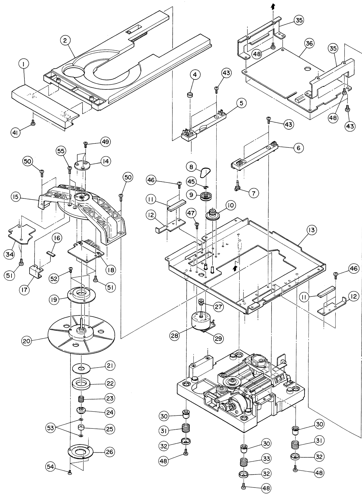
EXPLODED VIEW-3
