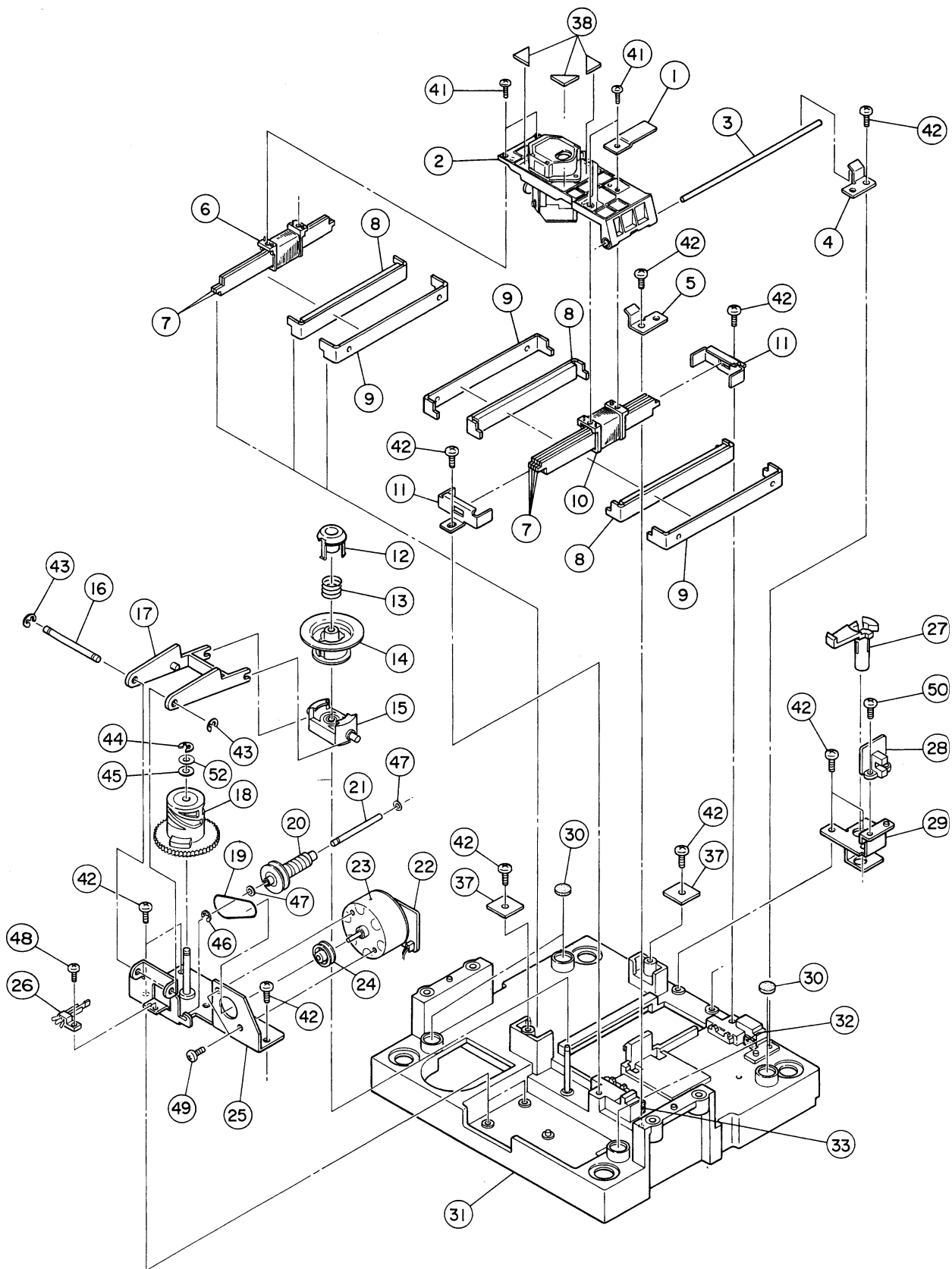
EXPLODED VIEW-4
