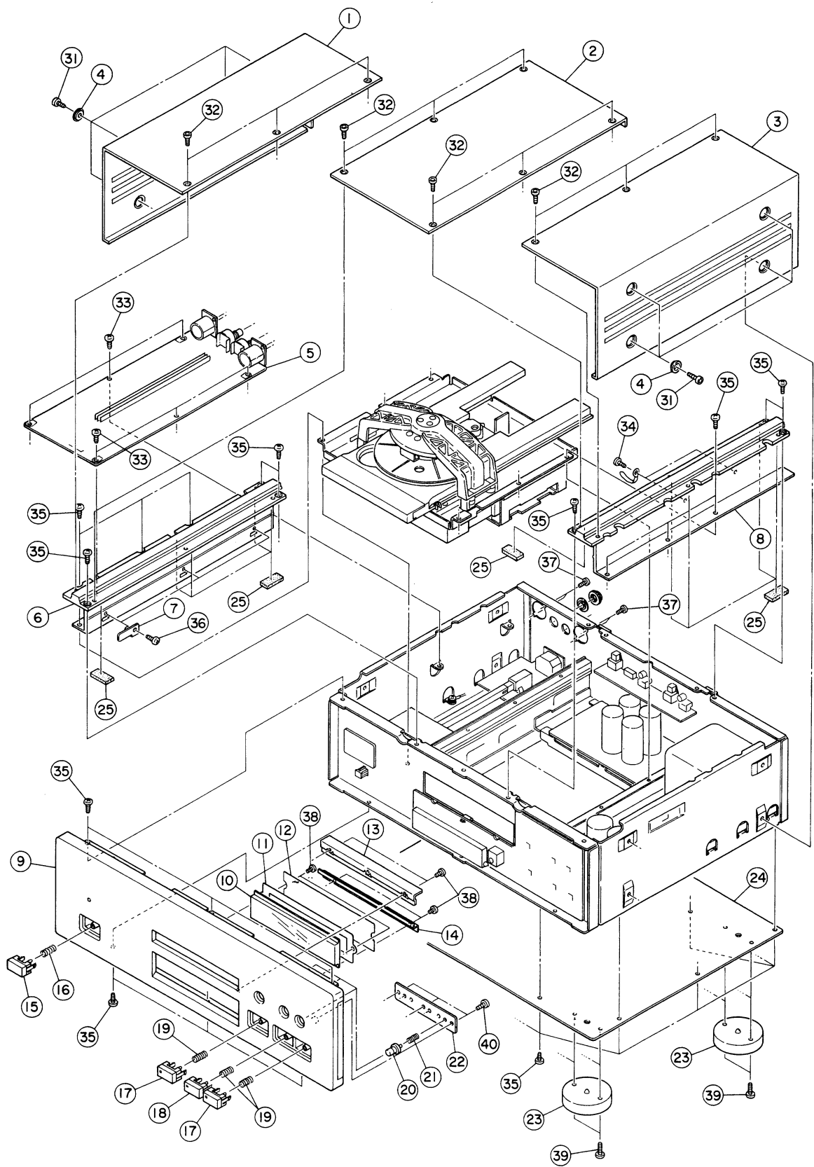
EXPLODED VIEW-1
