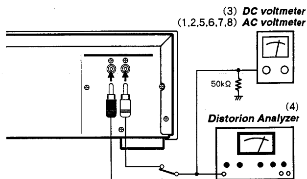
Fig. 4-6 Test setup
