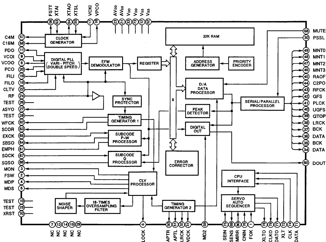
U403 CXD2500AQ
