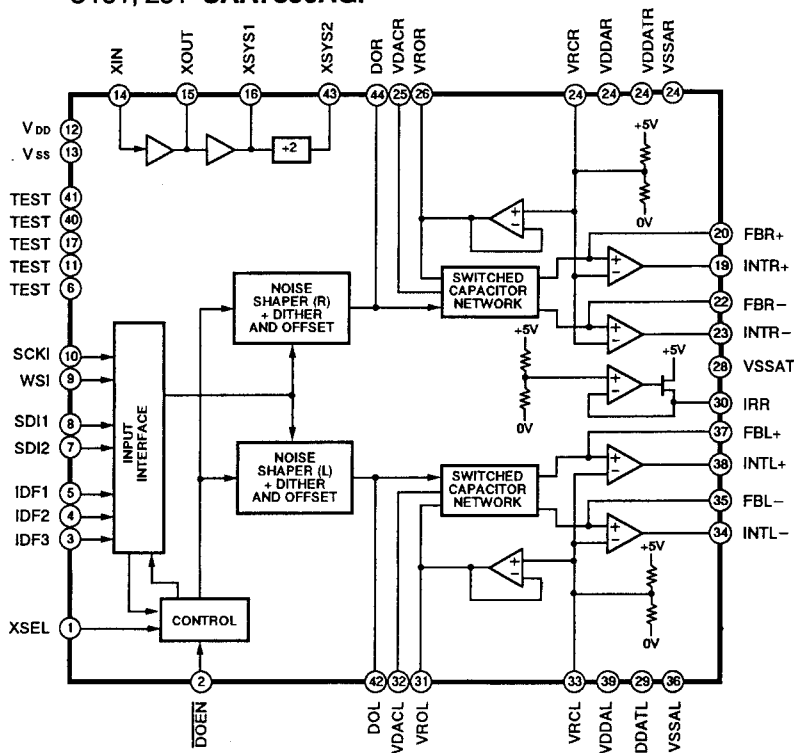
U151, 251 SAA7350AGP
