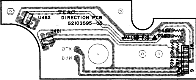
DIRECTION PCB
