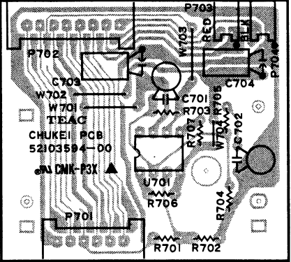
CHUKEI PCB
