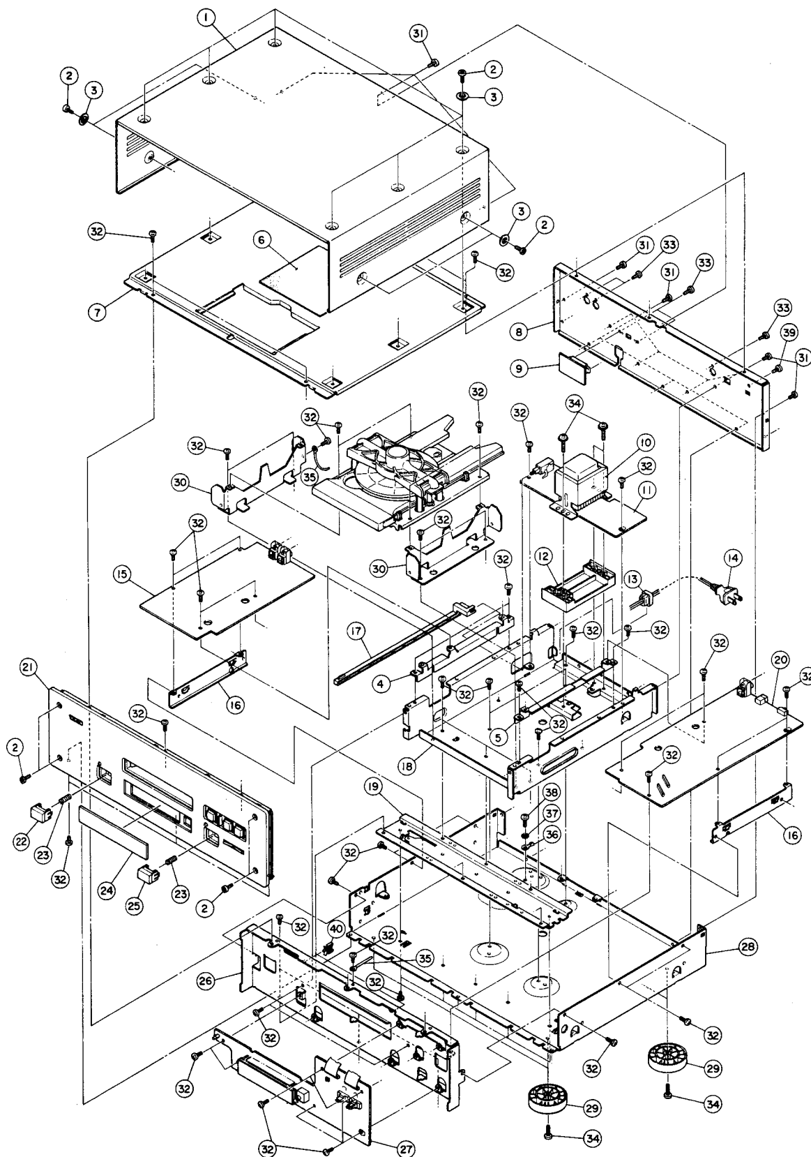
EXPLODED VIEW-1
