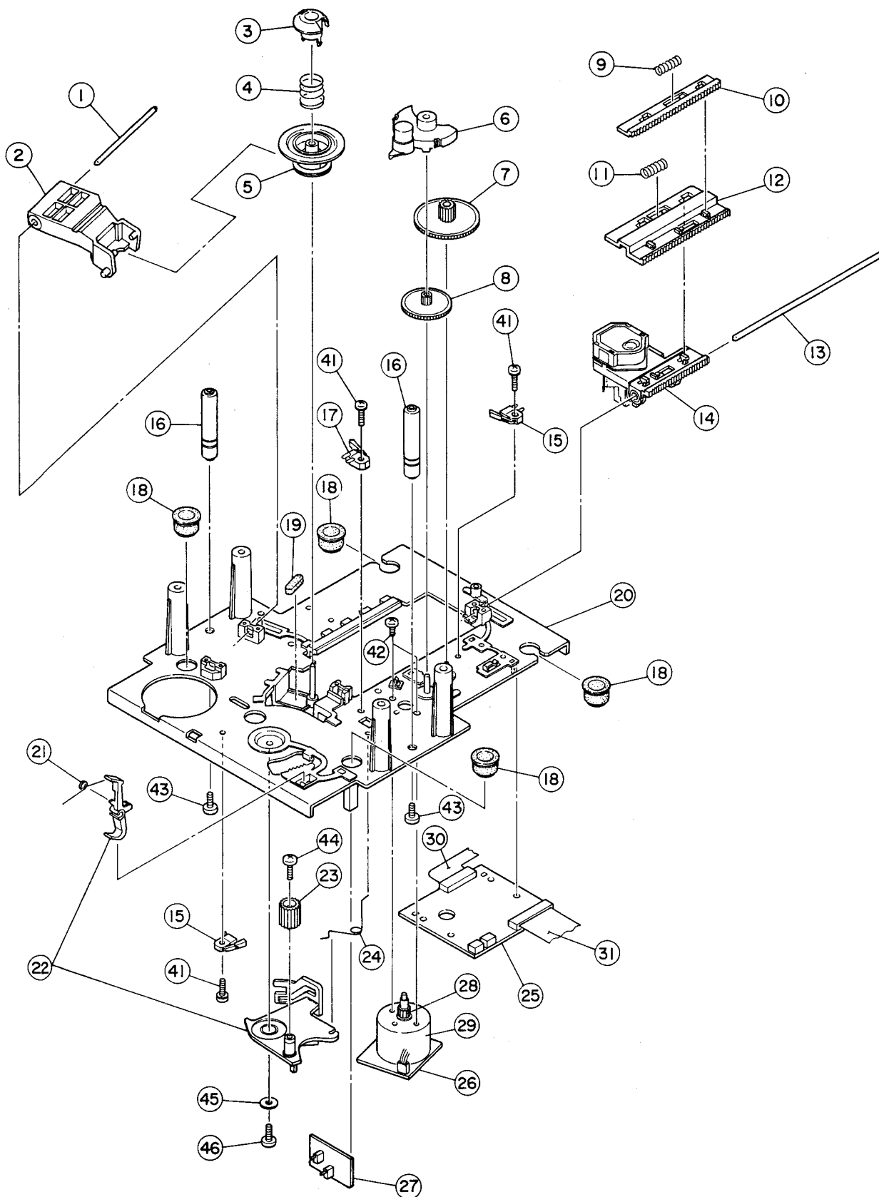
EXPLODED VIEW-3
