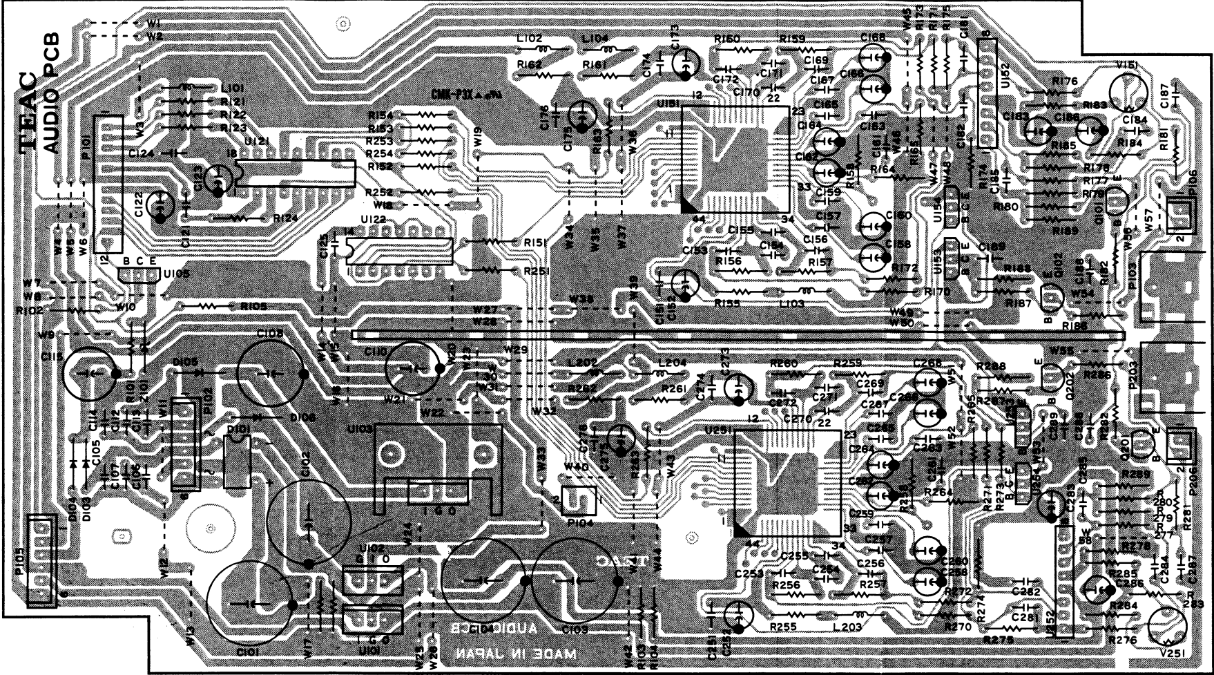
AUDIO PCB
