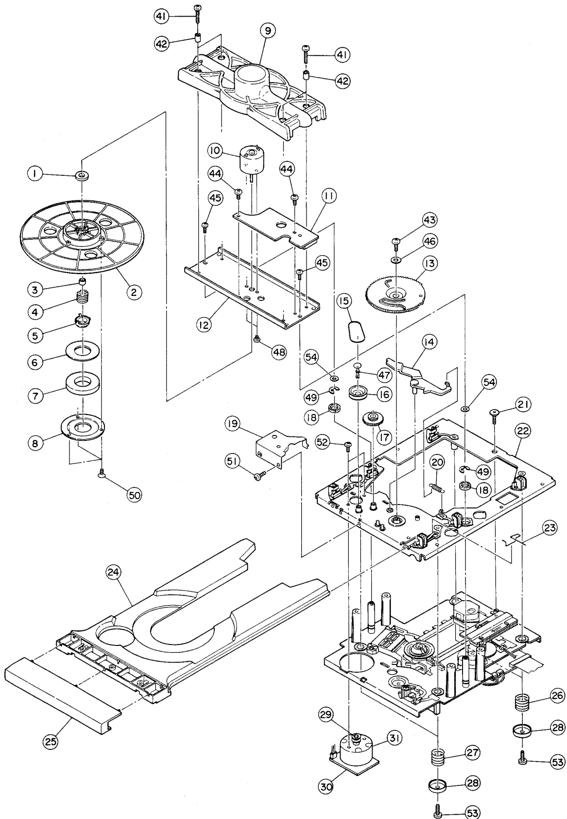
EXPLODED VIEW-2
