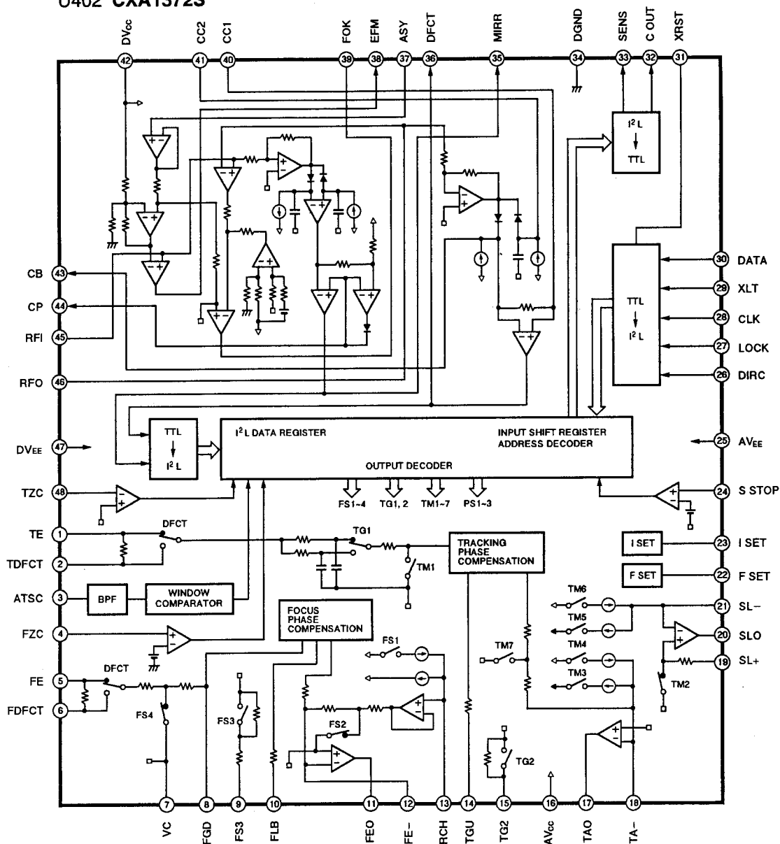
U402 CXA1372S
