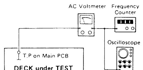
Fig. 5-5 Test setup for bias adjustment
