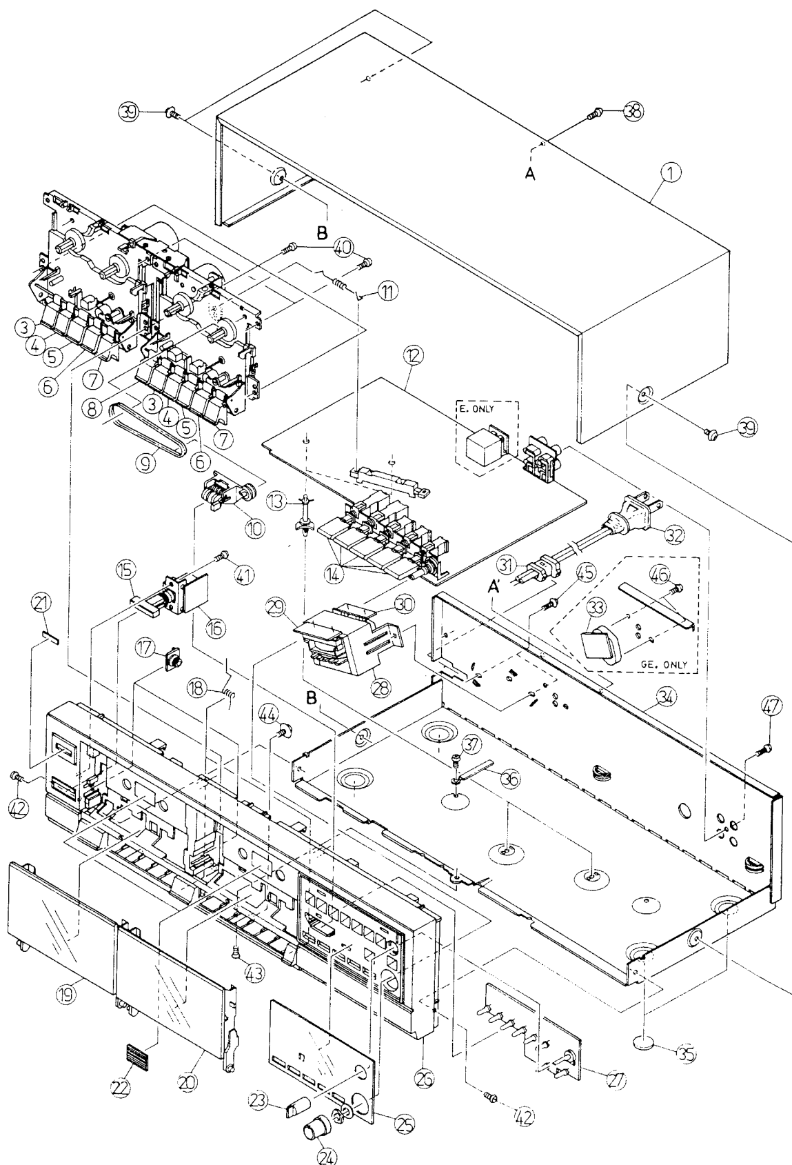
EXPLODED VIEW-1
