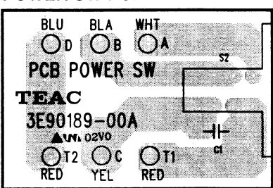
POWER SW PCB
