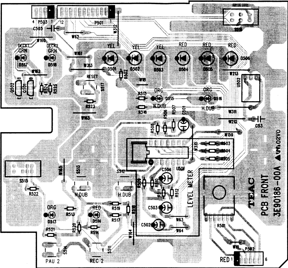
FRONT PCB
