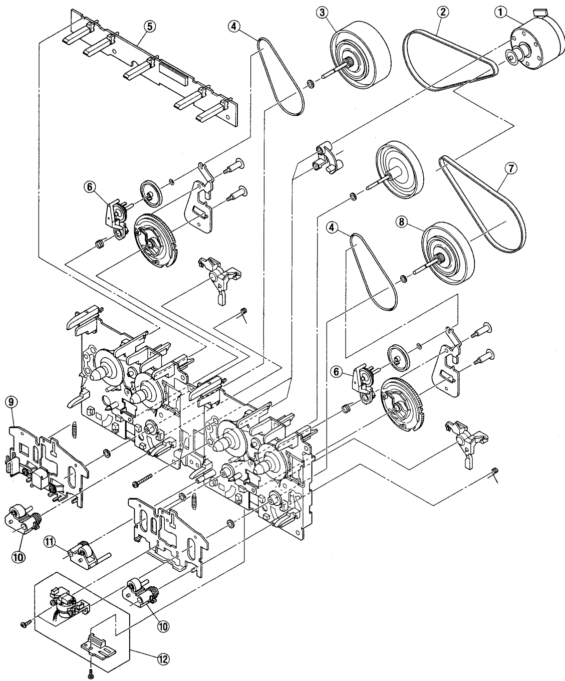
EXPLODED VIEW-2 (CMAT5Z026A)
