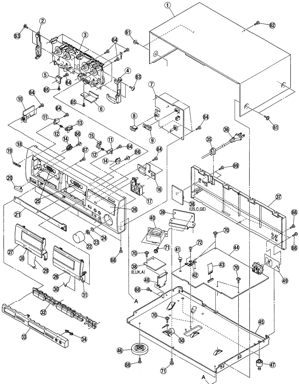
EXPLODED VIEW-1
