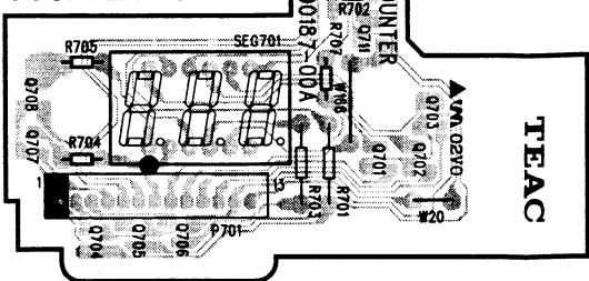
COUNTER PCB
