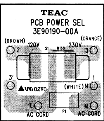
POWER SEL PCB
