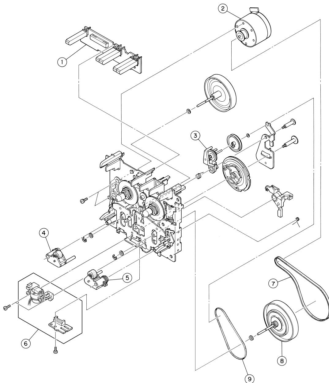
Exploded View-2
