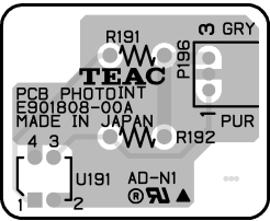
PHOTO INT PCB
