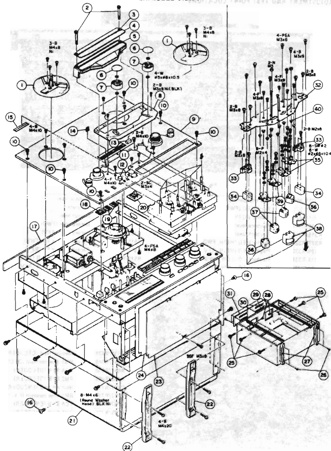
EXPLODED VIEW-1
