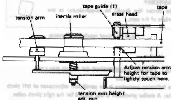
Fig. 2-21 Tension arm height adjustment
