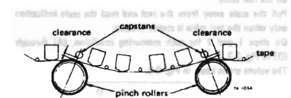
Fig. 2-4 Pause position and pinch roller pressure stroke adjustments
