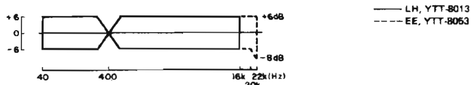
Fig. 3-10 Overall frequency responses with DBX IN (9.5cm/s)
