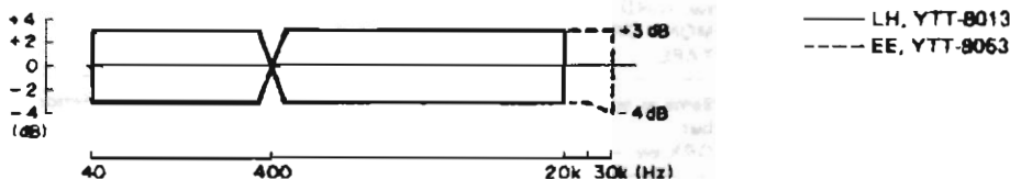
Fig. 3-7 Overall frequency responses (19cm/s)
