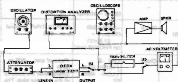
Fig. 3-1 Basic connection
