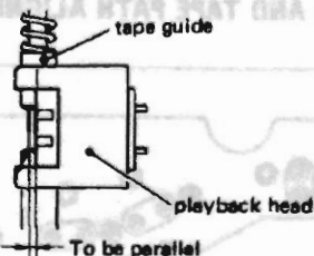
Fig. 2-19 Playback head tilt adjustment
