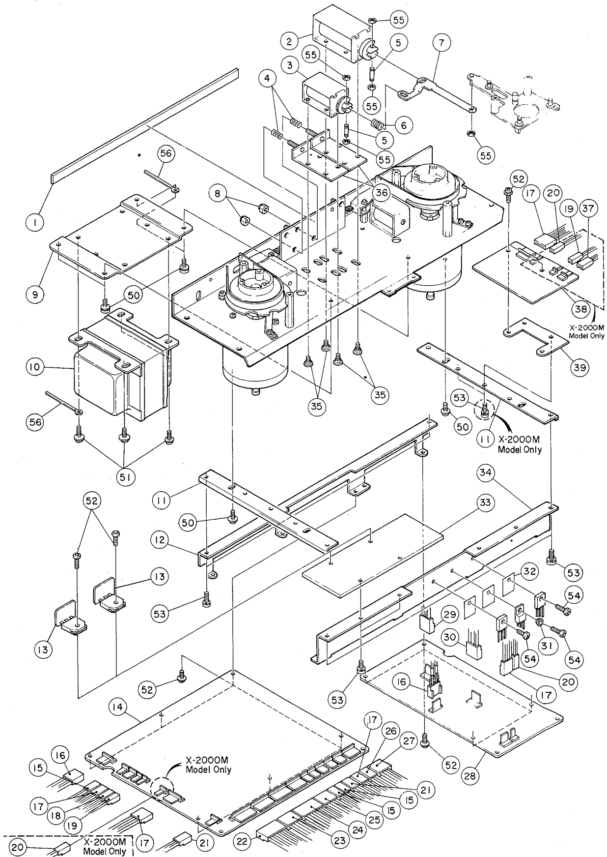
EXPLODED VIEW-4
