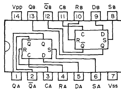
HD14013BP
