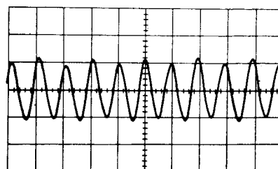
Fig. 3-13 RMS symmetry adjustment (correct) (RMSシンメトリ調整・良)
