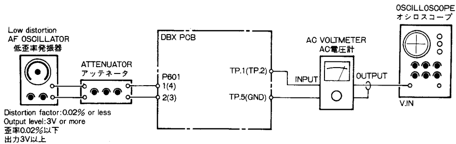
Fig. 3-14 RMS symmetry adjustment setup (decoder)
