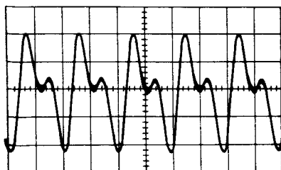
Fig. 3-12 RMS symmetry adjustment (incorrect) (RMSシンメトリ調整・不良)
