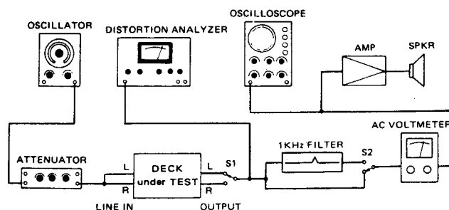
Fig. 3-3 Basic connection
