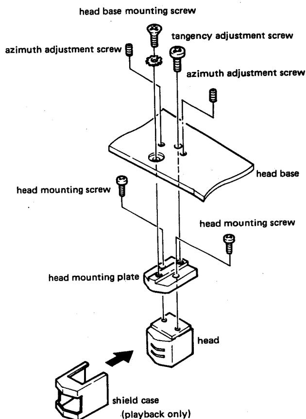
Fig. 2-23 Head mounting
