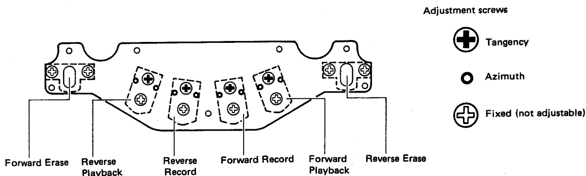
Fig. 2-21 Head arrangement
