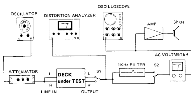
Fig. 3-1 Basic connection
