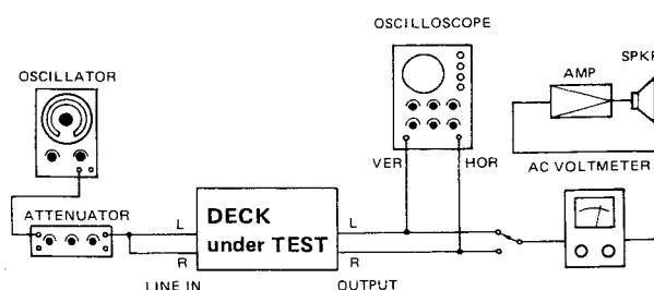
Fig. 3-2 Connection
