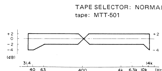
Fig. 6-8 Overall frequency response
