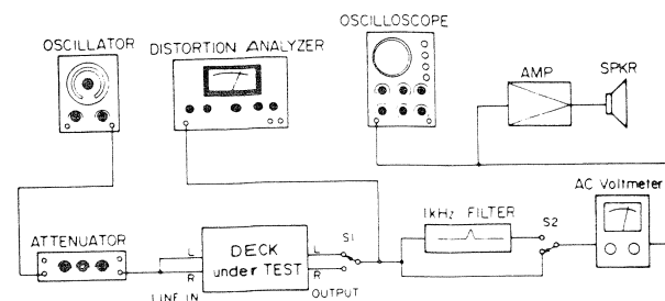
Fig. 6-1 Basic test setup
