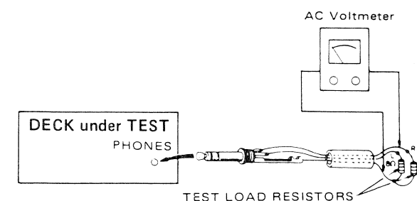
Fig. 6-10 Test setup for PHONES check
