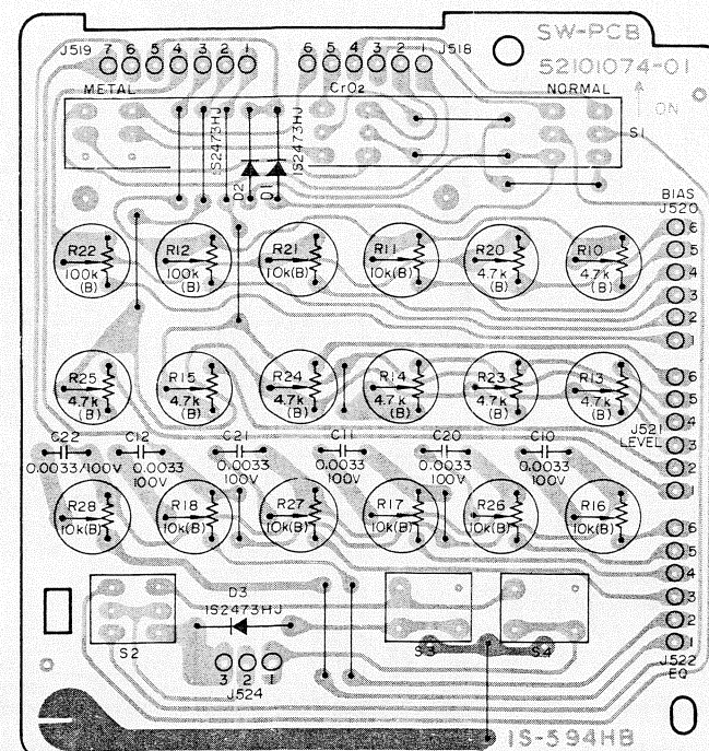
SWITCH PCB R ASSY
