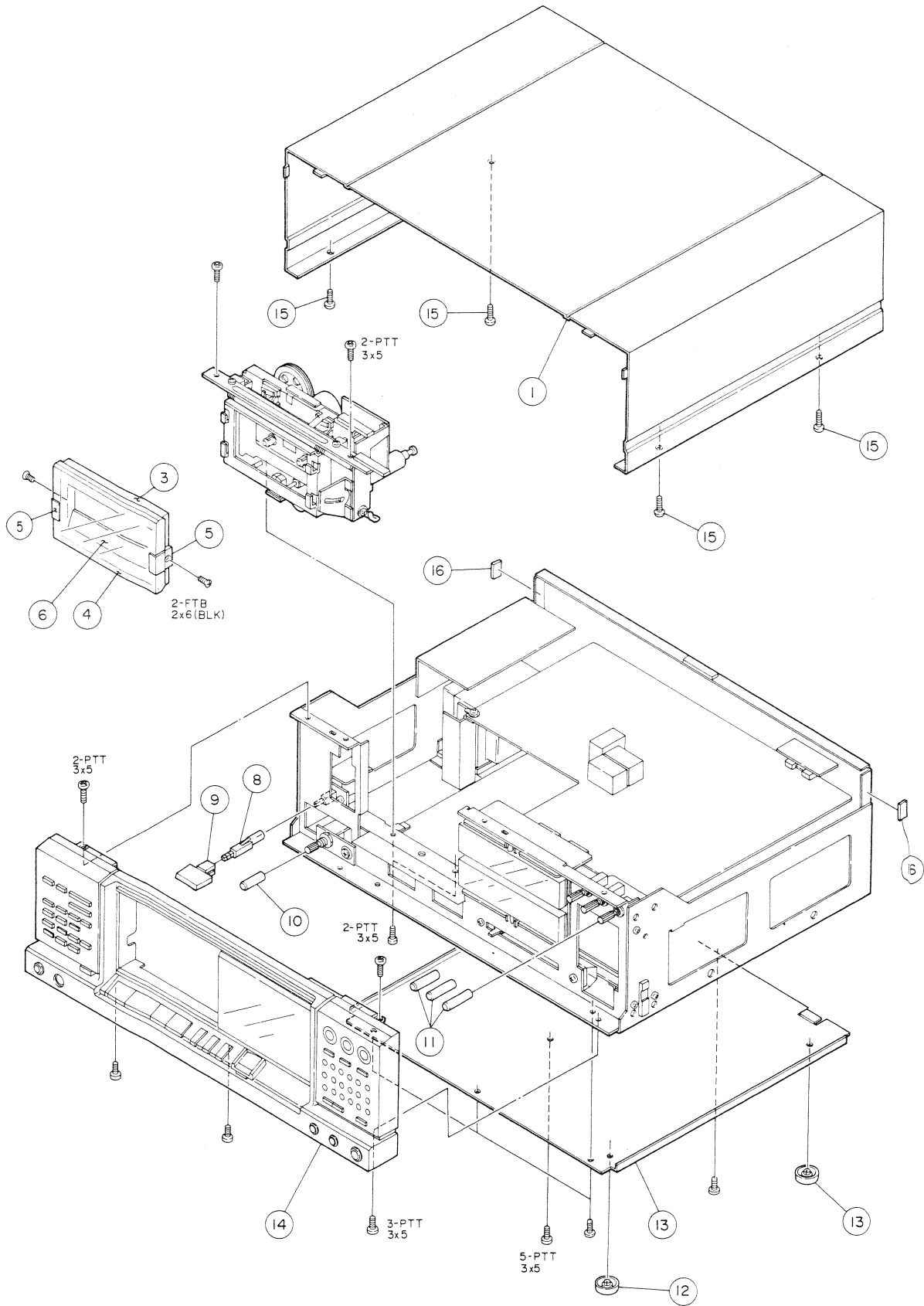
EXPLODED VIEW-1
