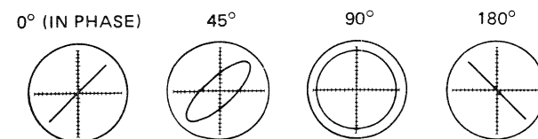
Fig. 6-4 Confirming phase relationship
