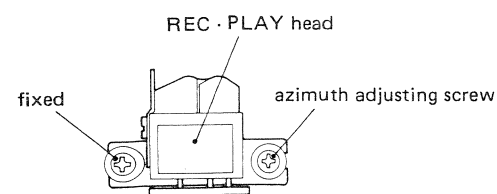
Fig. 6-3 Azimuth screw location
