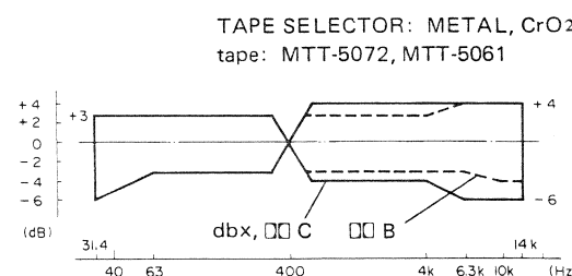
Fig. 6-7 Overall frequency response (NR IN)
