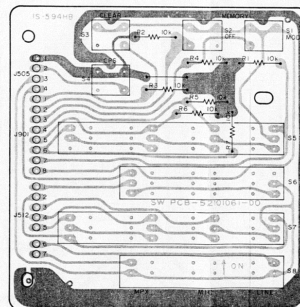
SWITCH PCB L ASSY
