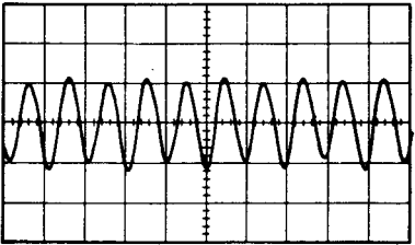
Fig. 6-16 RMS SYM check (Correct) (RMS SYM 良)
