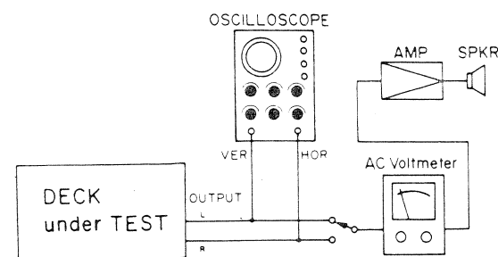
Fig. 6-2 Test setup for azimuth check
