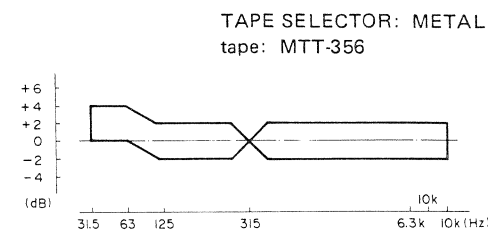
Fig. 6-5 Playback frequency response
