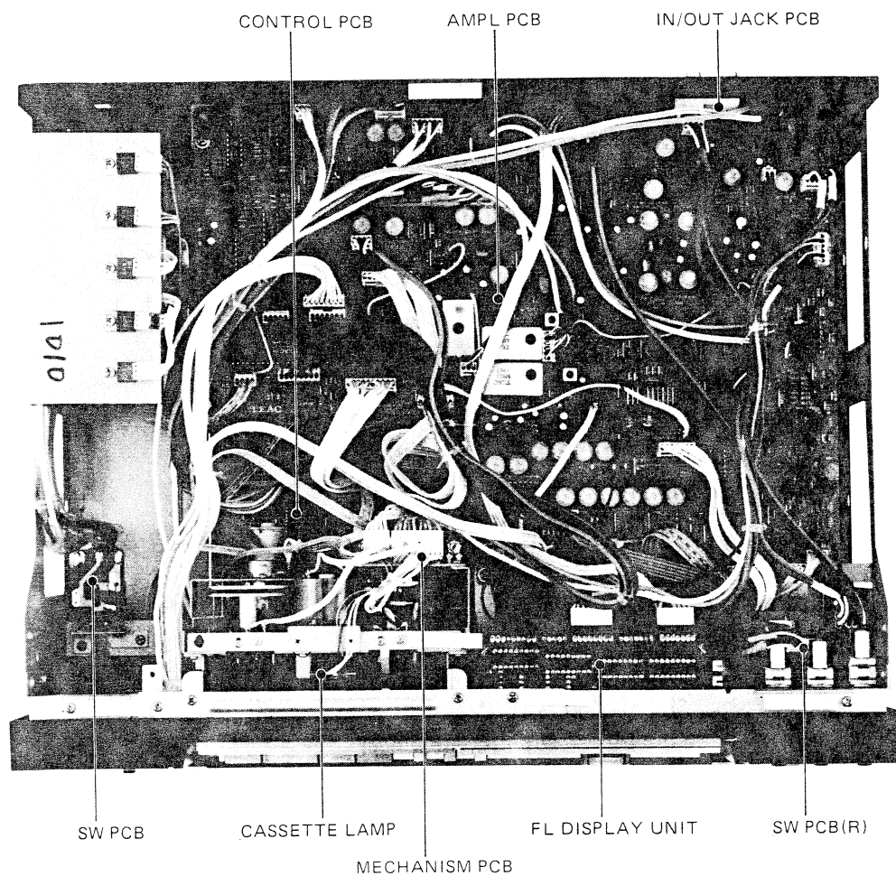
Fig. 3-1 Top view (上面)
