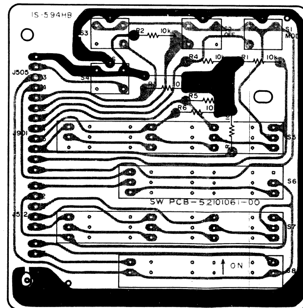
SWITCH PCB L ASSY
