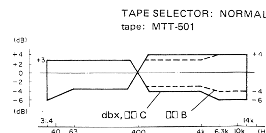
Fig. 6-9 Overall frequency response (NR IN)
