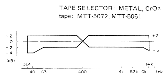
Fig. 6-6 Overall frequency response
