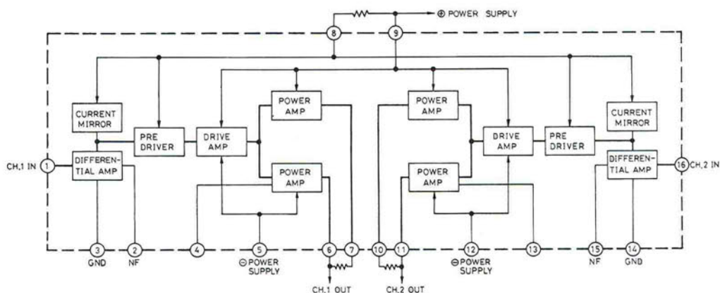
IC601 (SVISTK459) 2 Channel Power Amplifier
