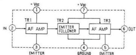
IC401, 402 (SVTA7129P) Equalizer Amplifier
