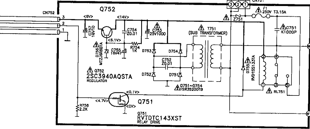
F POWER CIRCUIT ( P.C.Board on page 41 )
