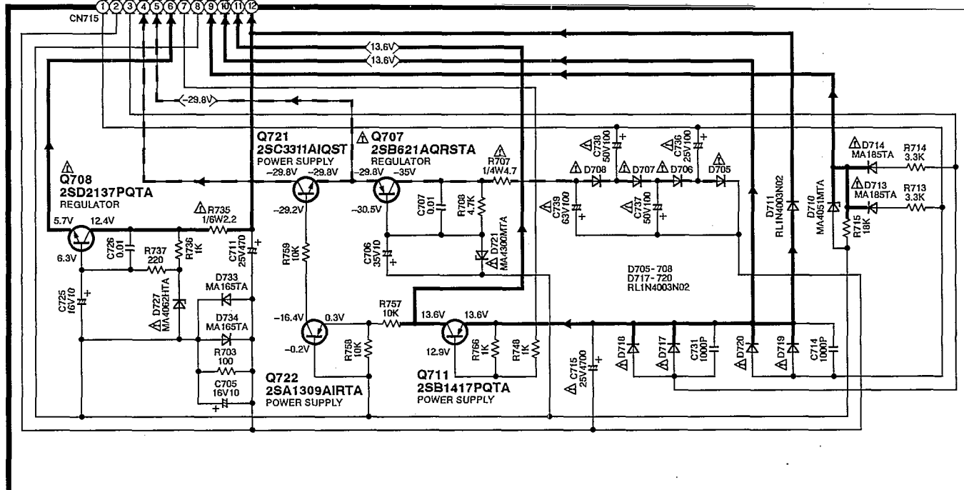
F POWER SUPPLY CIRCUIT (P.C. Board: on page 33)
