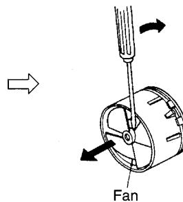
Step 2 Put a screwdriver at the root of the fan and remove it.
