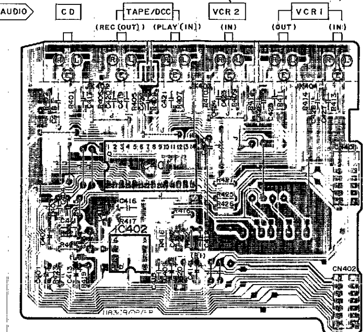
E IN/OUT TERMINAL P.C.B. (REP1732C-P... (E,EB) REP1732D-P... (EG) REP1732E-P... (G) REP1732F-P... (GN)
