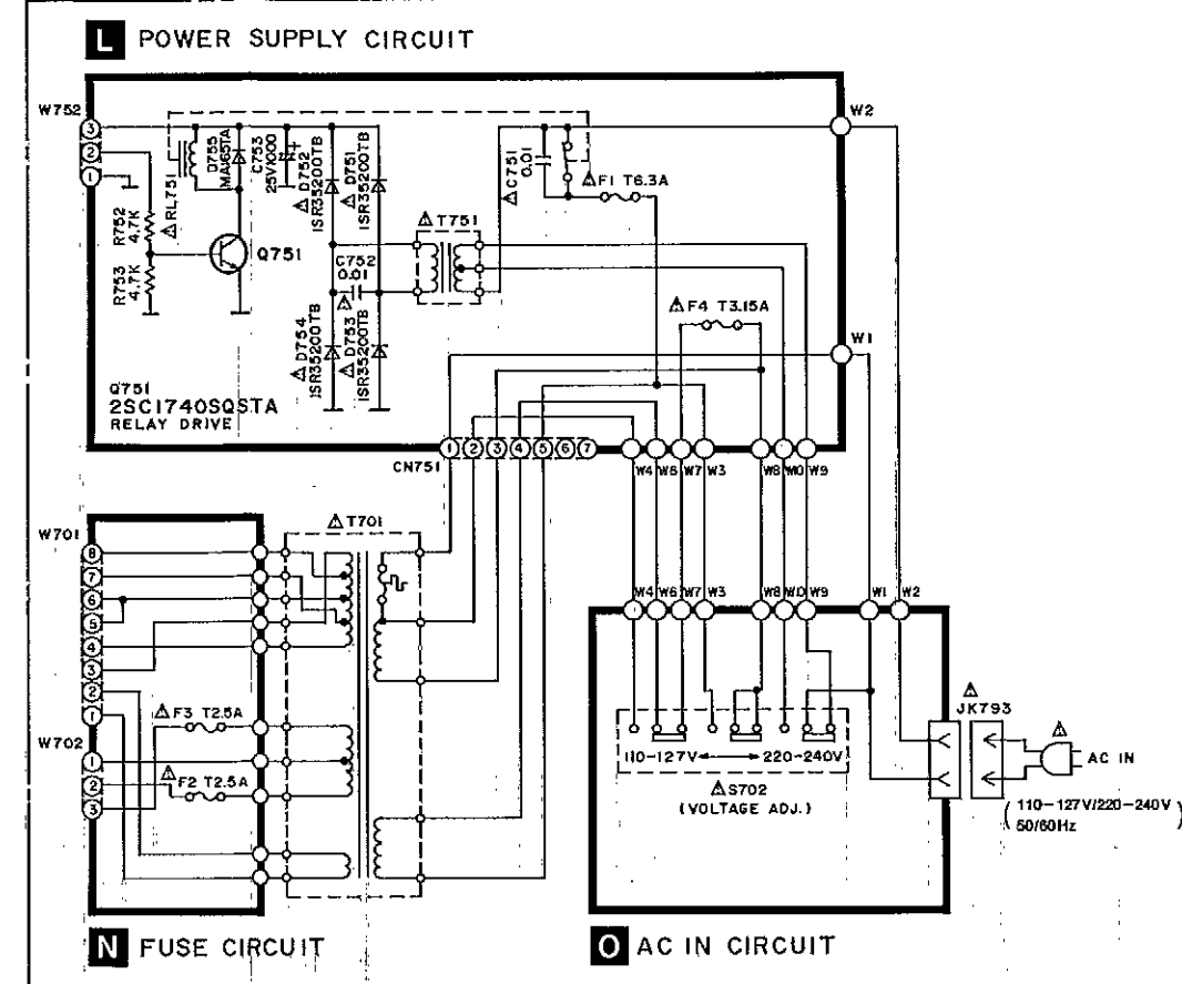
Power Source Circuit For [G] area.
