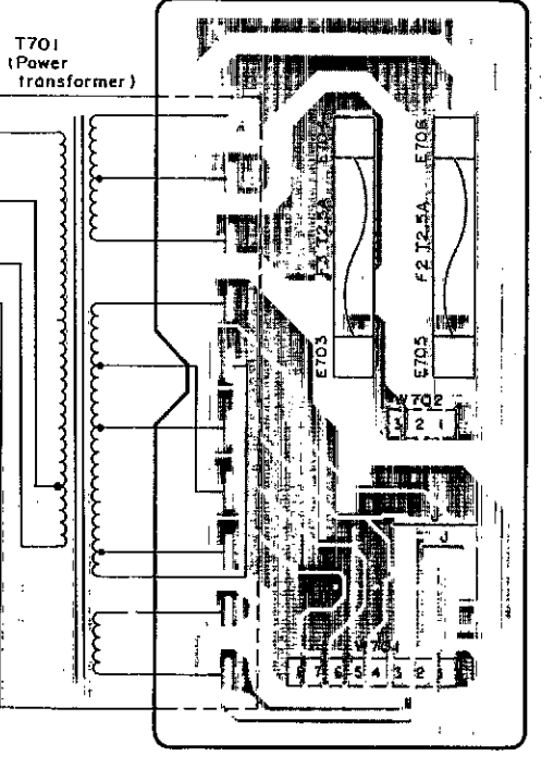
N FUSE P.C.B. For [E,EB,EG] areas. (REP1364B-M)
