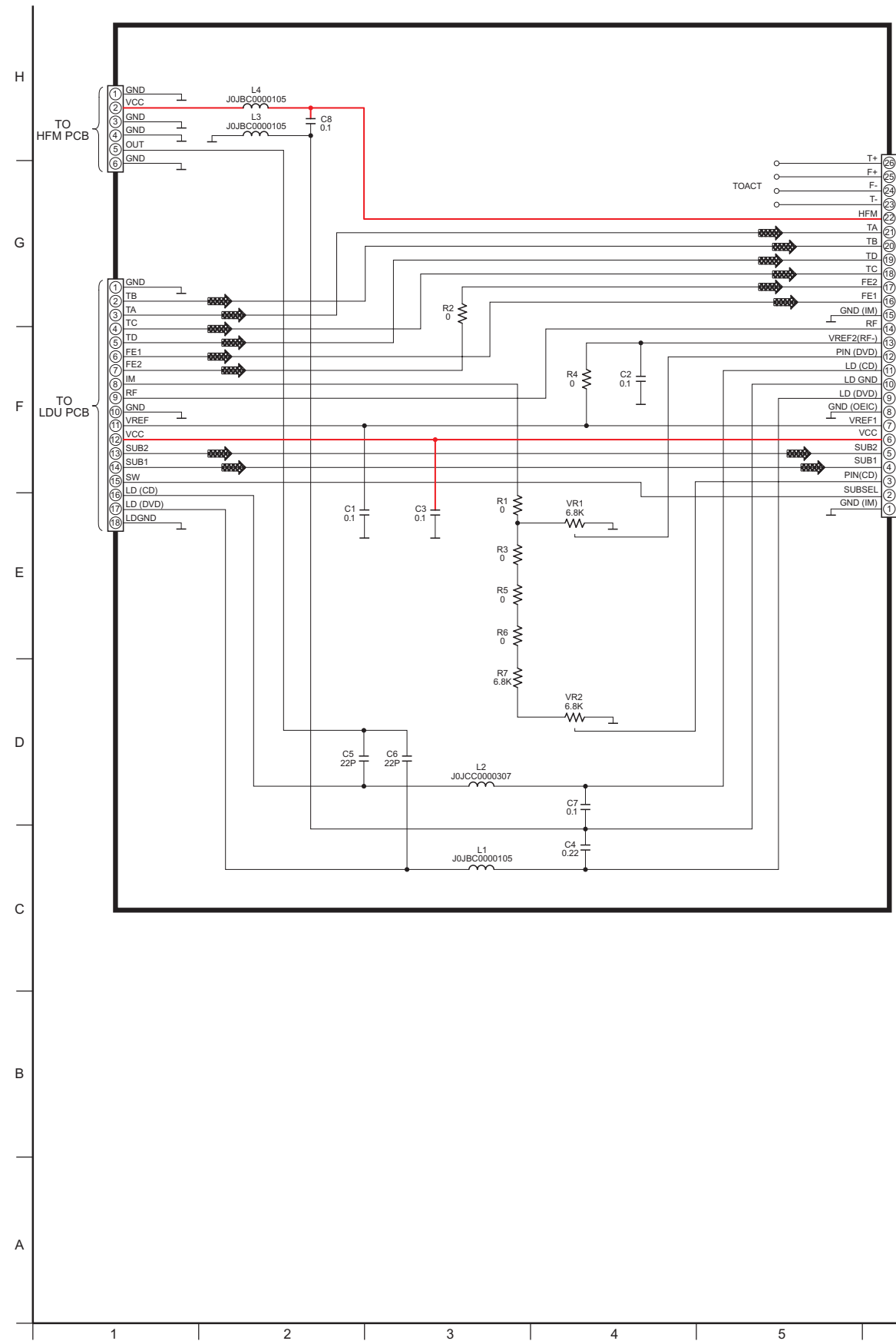
SCHEMATIC DIAGRAM-1 OPTICAL PICKUP UNIT CIRCUIT
