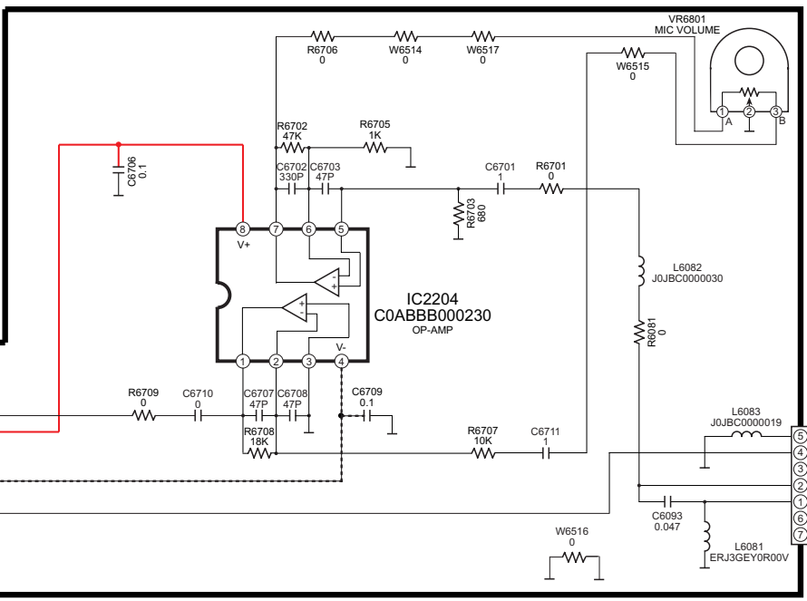
SA-HT340GC/GCS/GS MAIN/FL/VOLUME/MIC CIRCUIT
