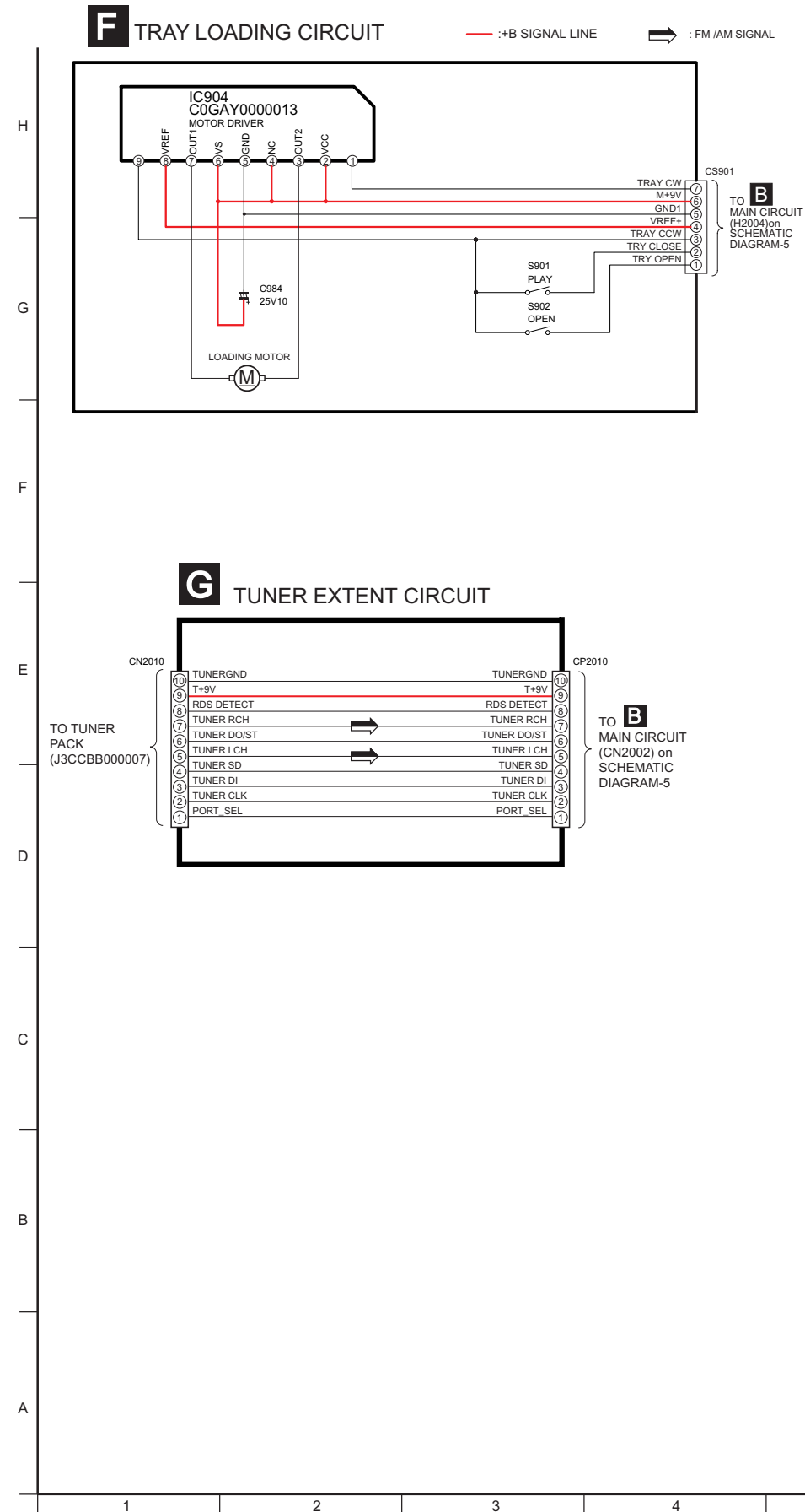
SCHEMATIC DIAGRAM-11
